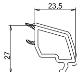
Parclose ref. 107.129
