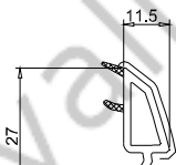
Parclose ref. 107.127
