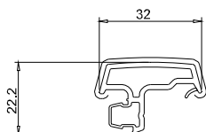
Battue ref. 109.680
