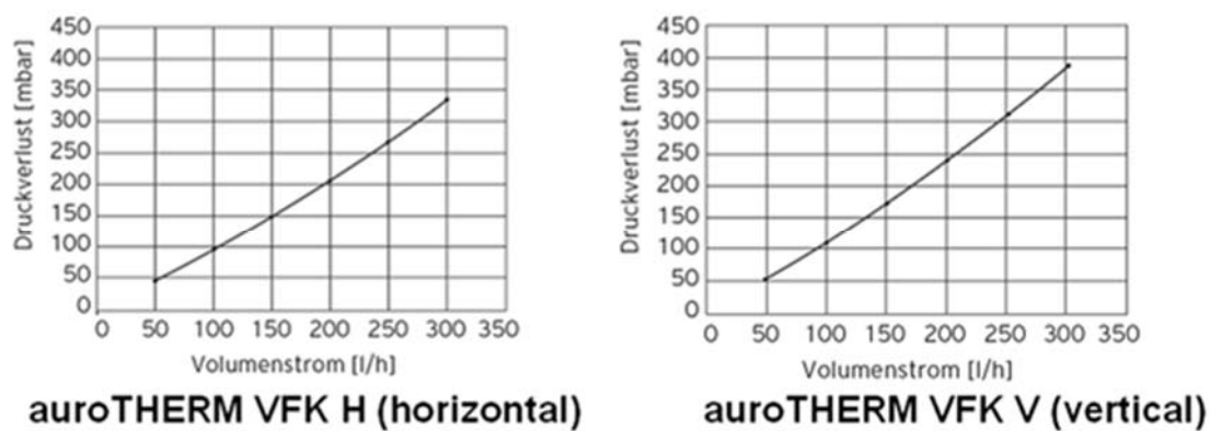
Figure 1 – Pertes de charge
