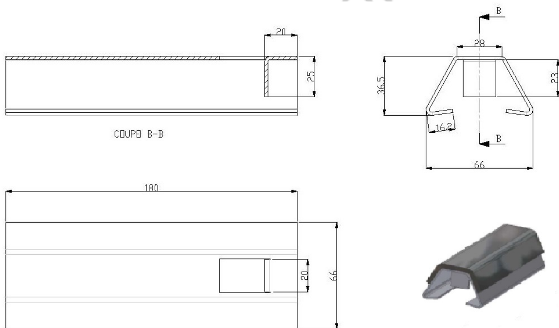
Figure 8 – Rehausse inférieure (Brevet FR1005097)
