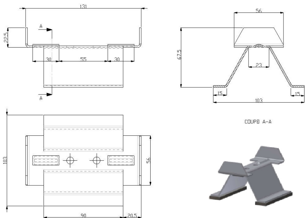
Figure 8 – Rehausse inférieure (Brevet FR1005097)
