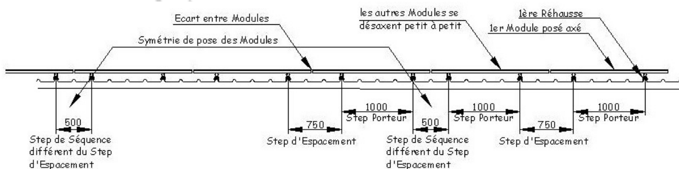
Figure 26 – Calepinage des rails
