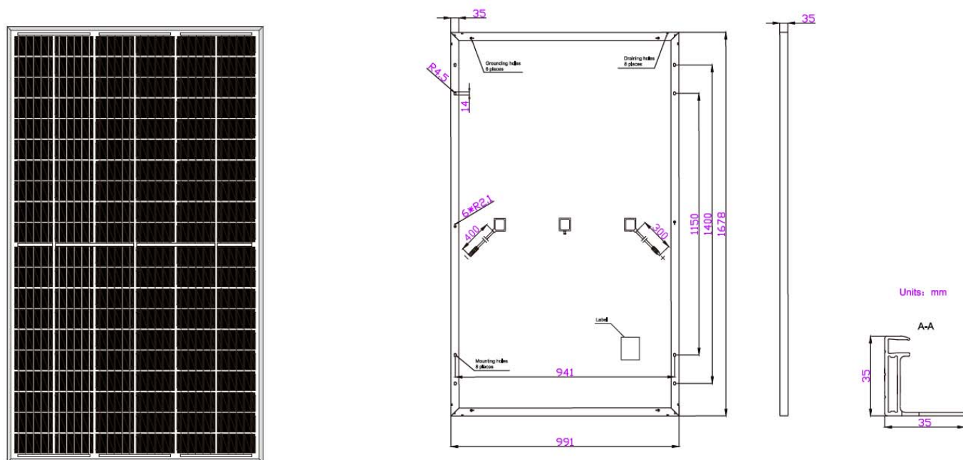
Figure 7 – Modules photovoltaïques et cadre : JAP60S03-XXX/SC
