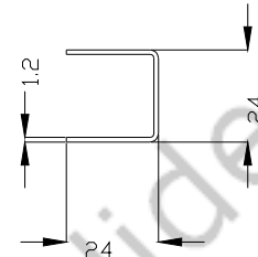
AP527 I_{yy} = 0.50 \text{ cm}^4 I_{xx} = 0.83 \text{ cm}^4
