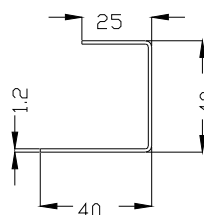
AP526 I_{yy} = 1.66 \text{ cm}^4 I_{xx} = 3.30 \text{ cm}^4
