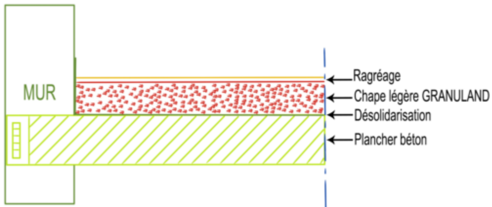
Figure 3 – Support plancher béton
