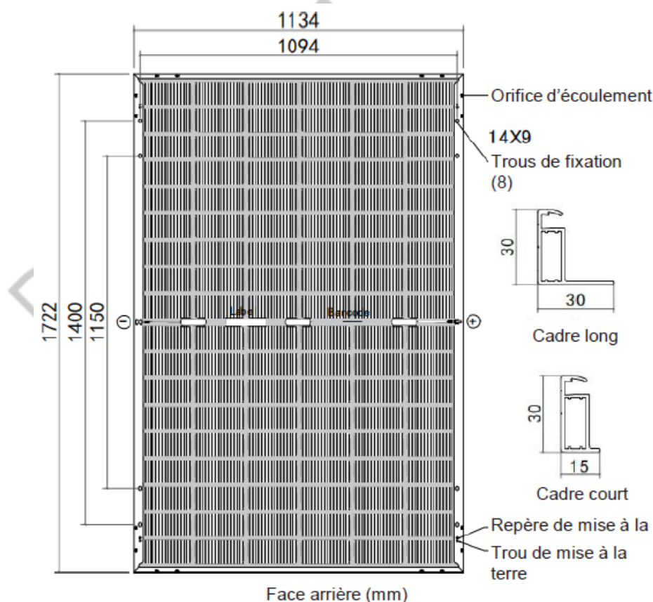
Modules DMEGC DMxxxM10T-B54HSW/HBW/HBB/HST/HBT
