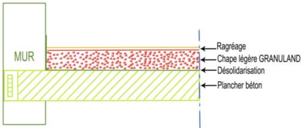
Figure 3 – Support plancher béton
