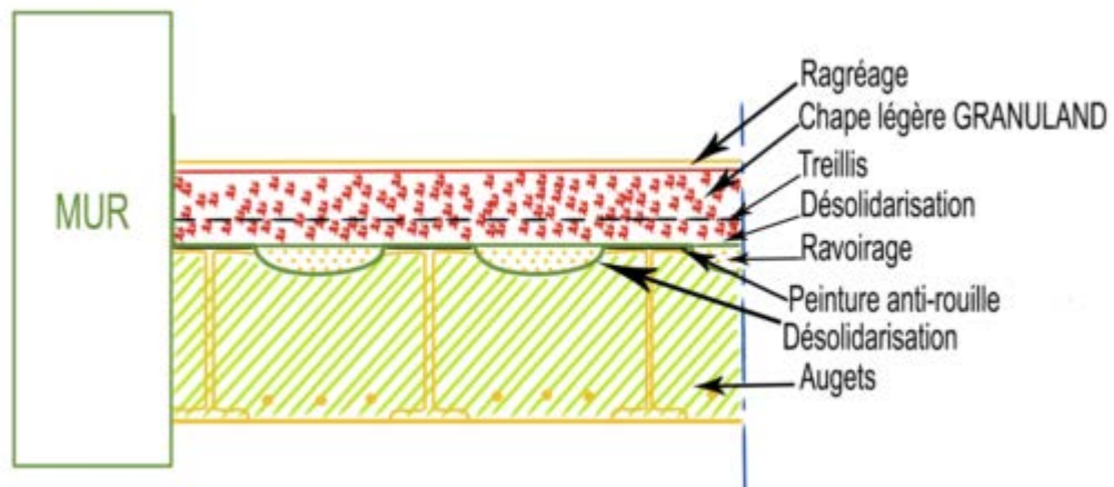
Figure 4 – Support plancher à augets
