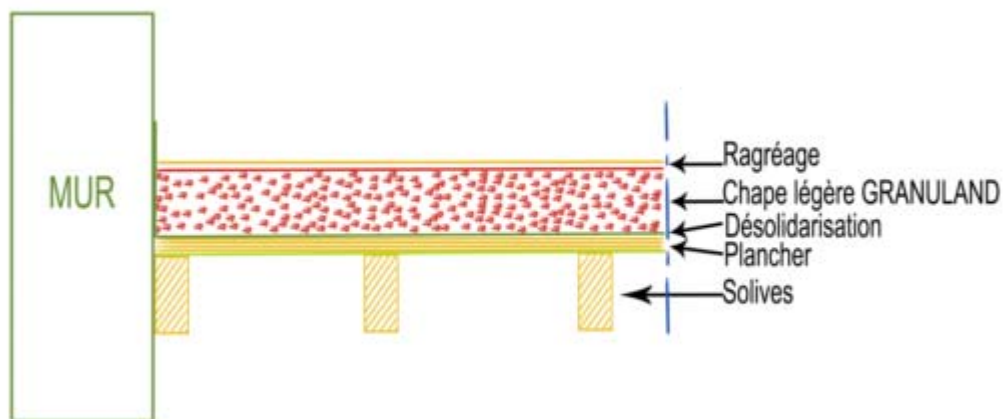
Figure 2 – Support plancher bois
