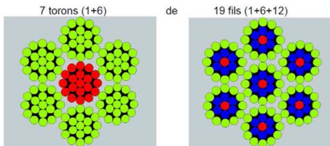
Figure 1 – Câble acier
