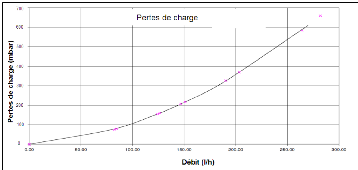
Figure 1 – Pertes de charge.
