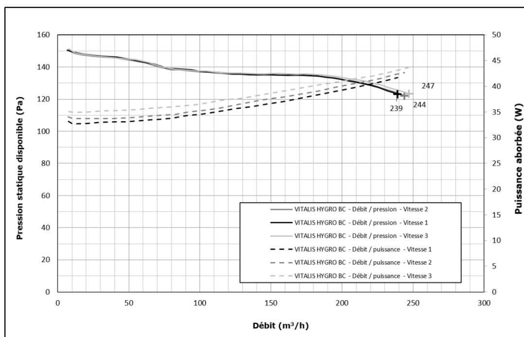
Figure 44 – VITALIS HYGRO BC
