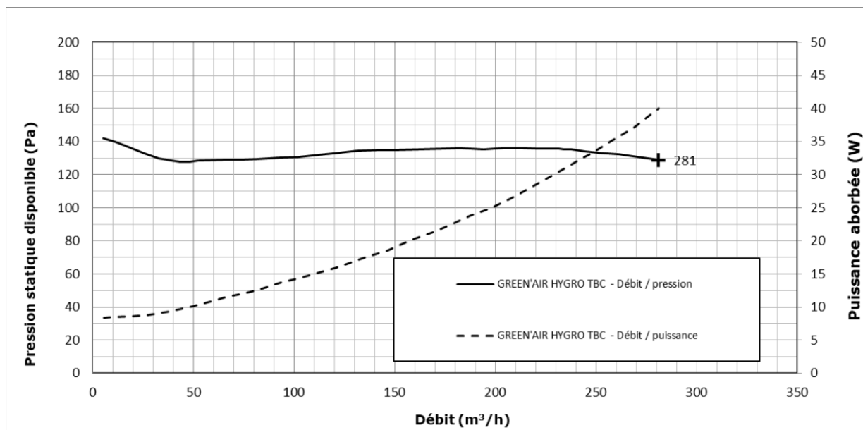
Figure 41 – GREEN'AIR HYGRO TBC
