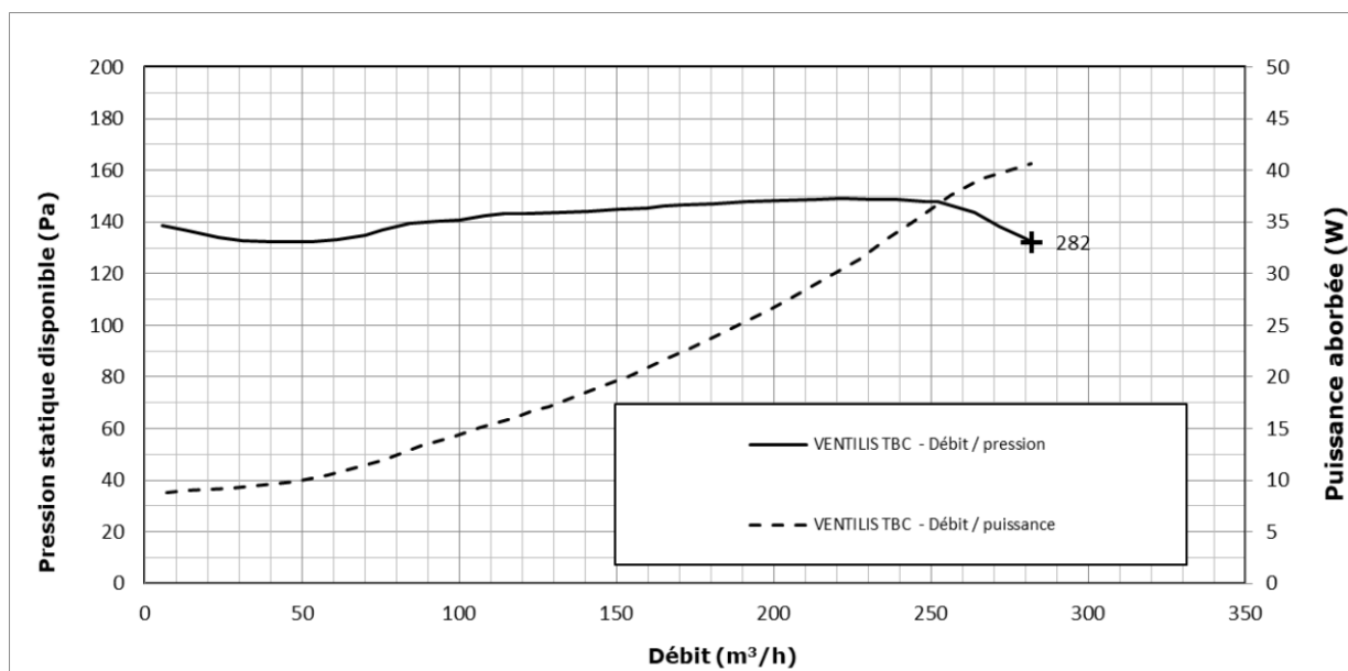
Figure 42 – VENTILIS TBC
