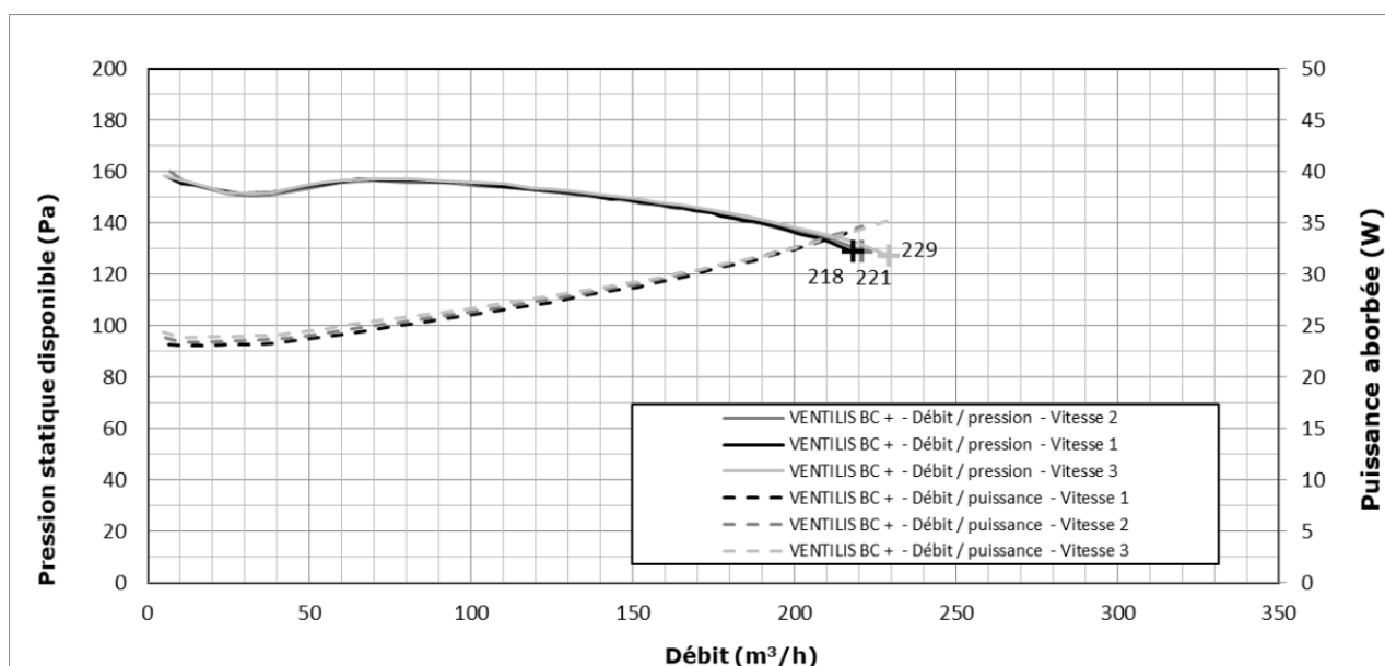
Figure 43 – VENTILIS BC+
