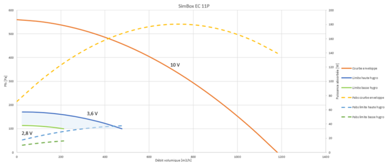
Figure 66 –SimBox EC 11P
