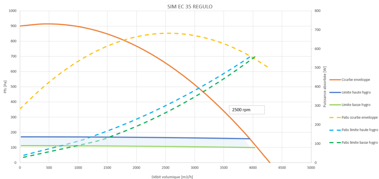
Figure 50 – SIM EC REGULO 35
