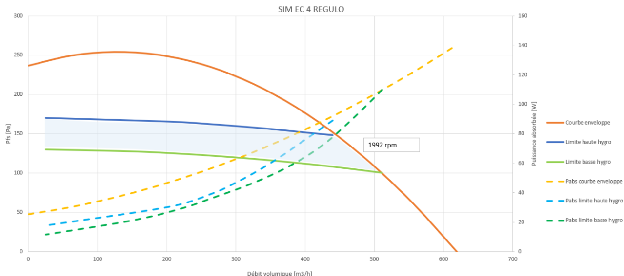
Figure 44 – SIM EC REGULO 4
