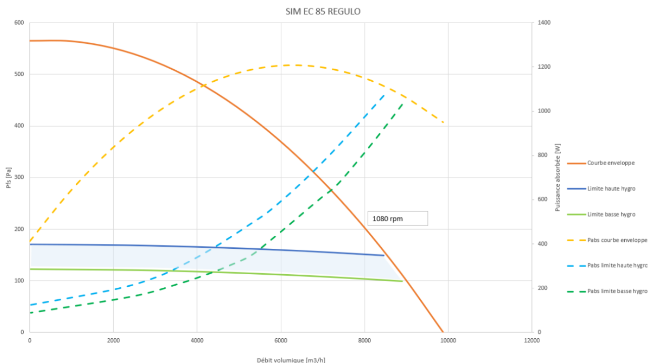
Figure 54 – SIM EC REGULO 85
