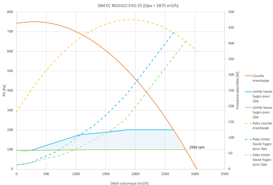
Figure 59 – SIM EC REGULO EVO 25
