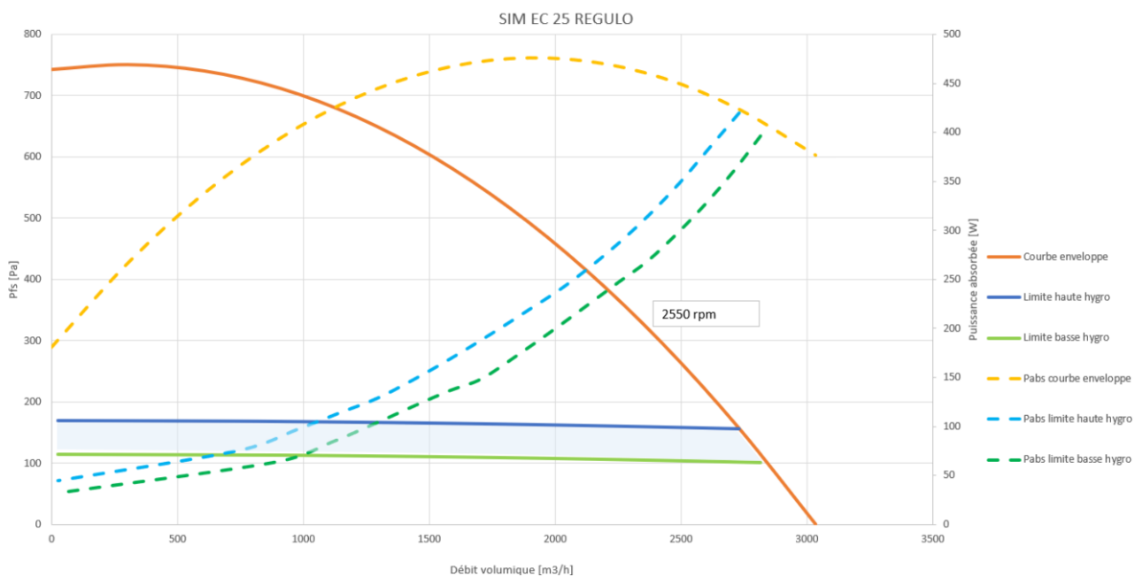
Figure 49 – SIM EC REGULO 25
