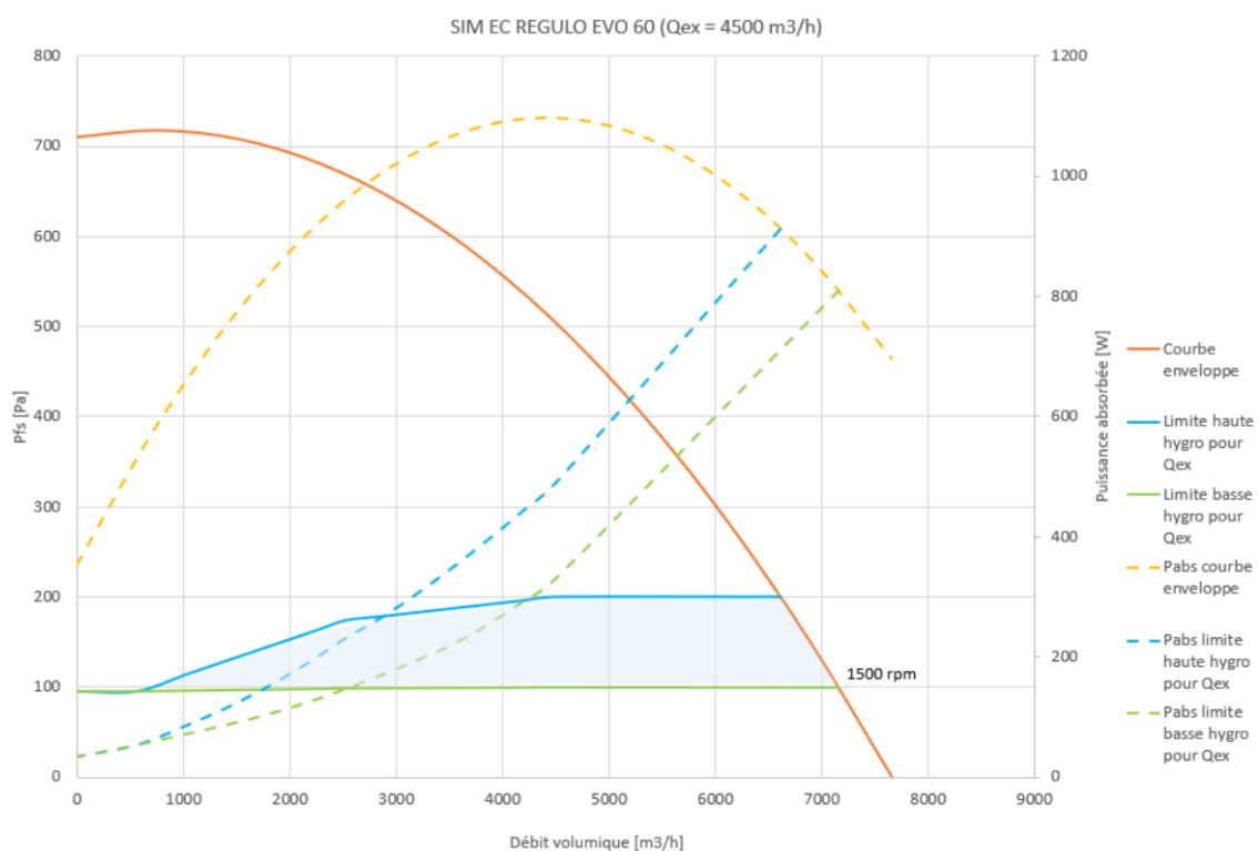
Figure 62 – SIM EC REGULO EVO 60
