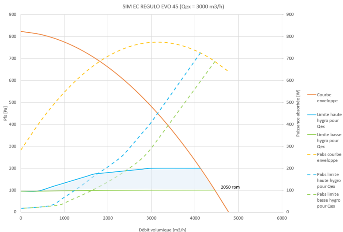
Figure 61 – SIM EC REGULO EVO 45
