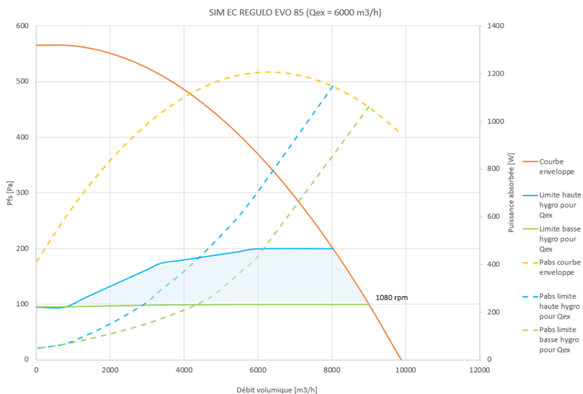
Figure 64 – SIM EC REGULO EVO 85
