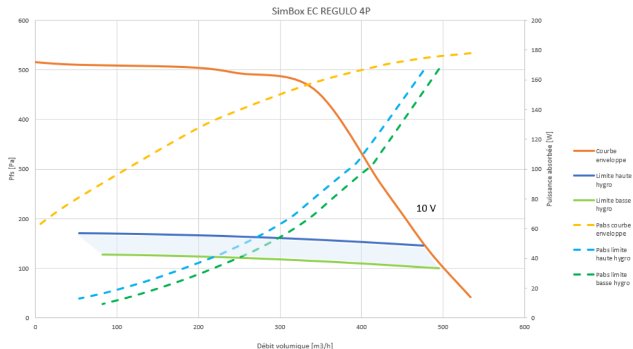
Figure 68 –SimBox EC REGULO 4P
