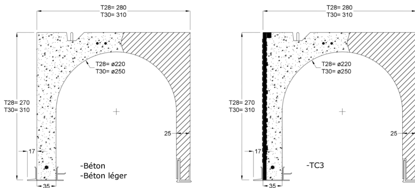
Figure 1 – Coffre PERFECTO Gen1 T28 et T30
