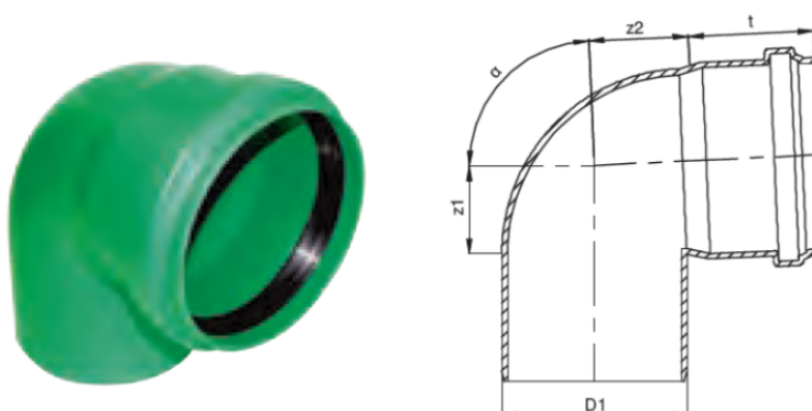
Figure 3.1 : Coudes MF
