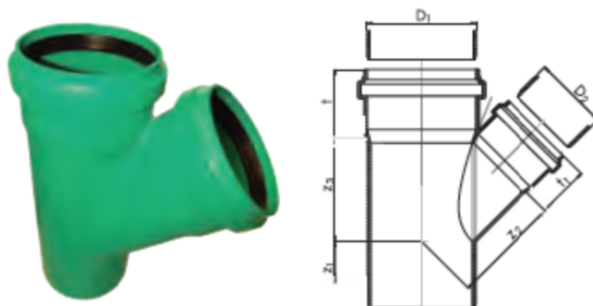
Figure 3.2 : Culottes MF 45°
