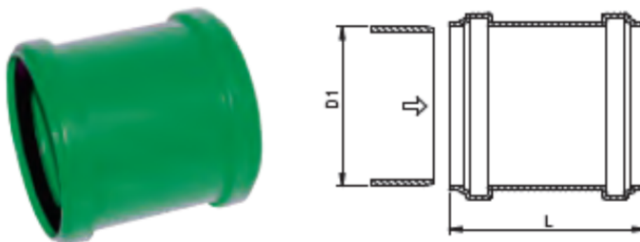
Figure 3.5 : Manchons
