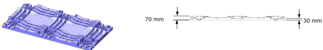
Figure 2a - Plaque de fond
