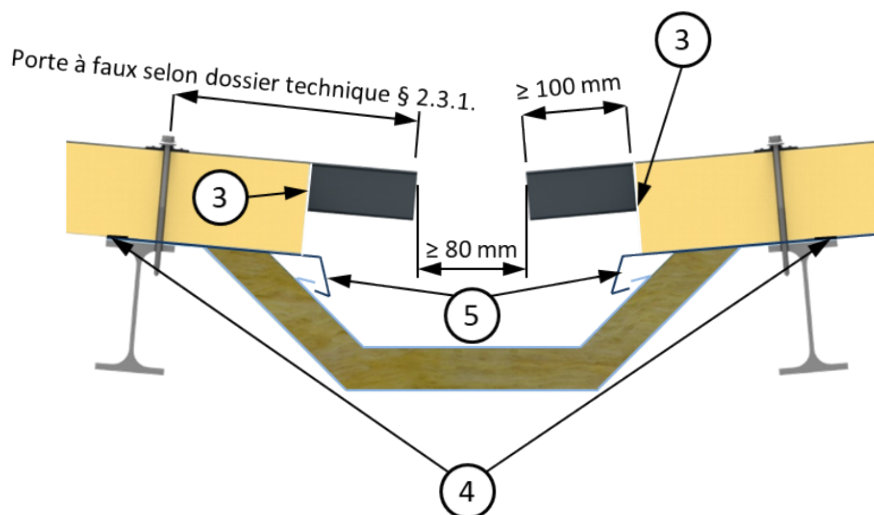
Figure 23 - Chéneau central
