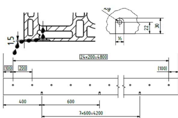
Figure 47 ter – EASY GLASS PRIME F
