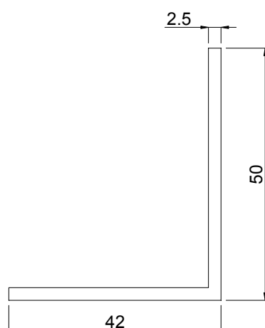
Figure 25 – Aboutage profilés TSP 203
