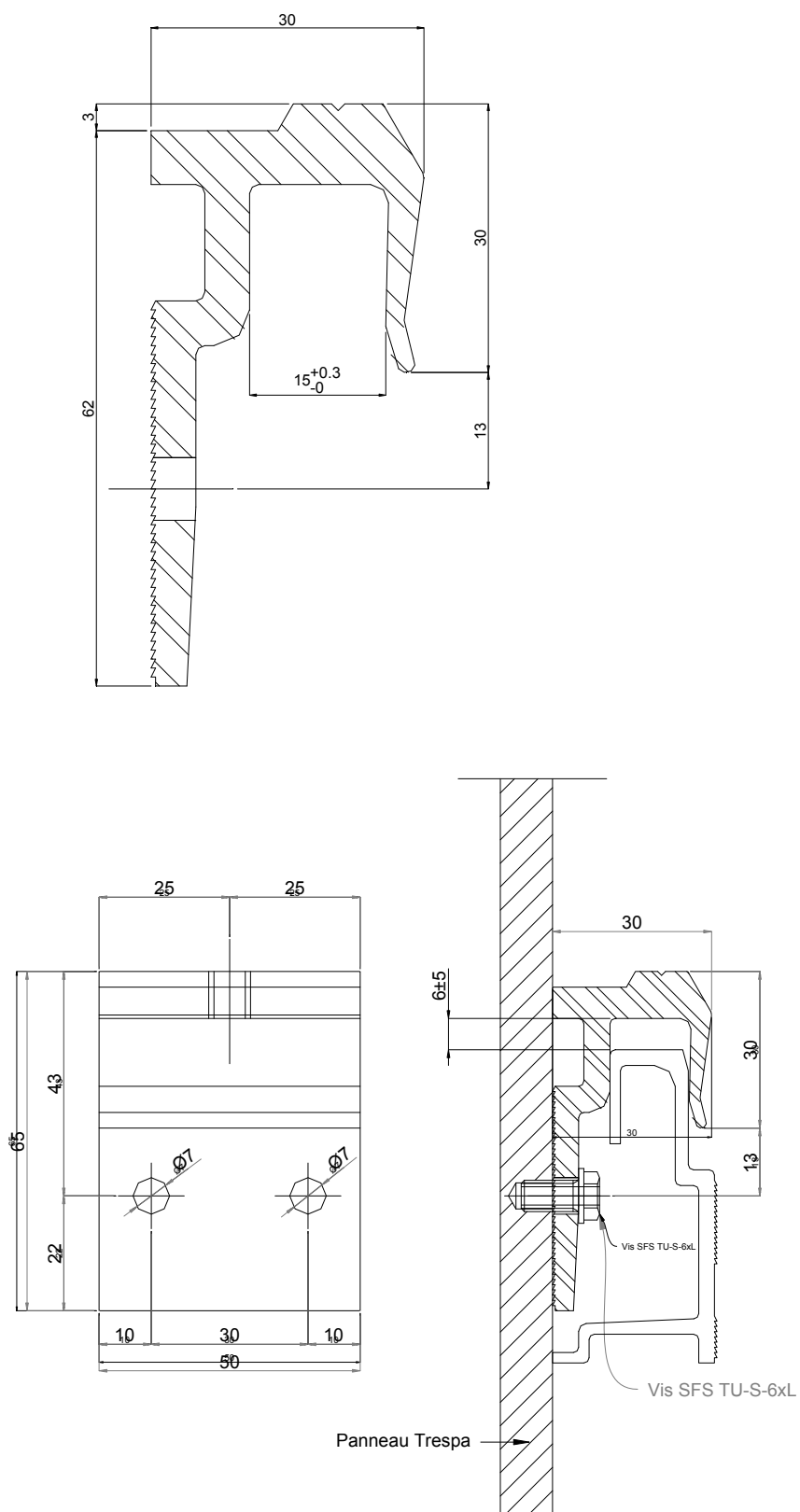
Figure 2 – Patte-agrafe TSP 204 standard sans taraudage
