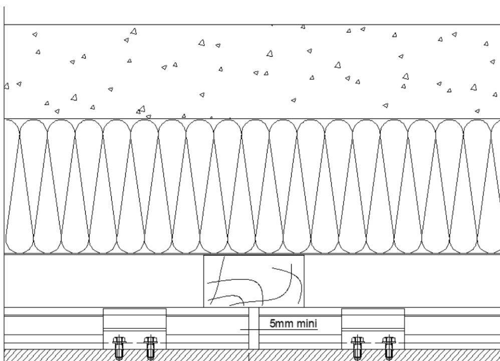
Figure 25 – Aboutage profilés TSP 203
