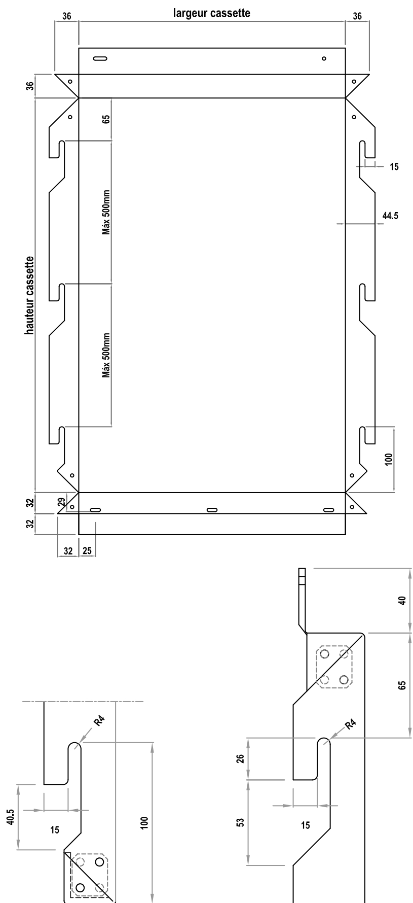
Figure 2b – Cassette 4 plis – type 1
