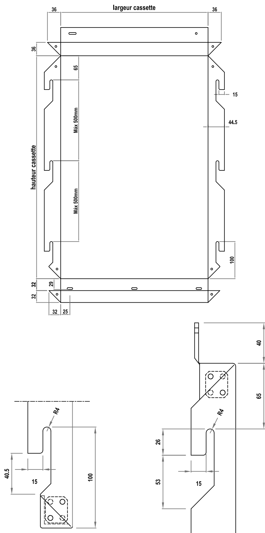
Figure 2c – Cassette 4 plis – type 2
