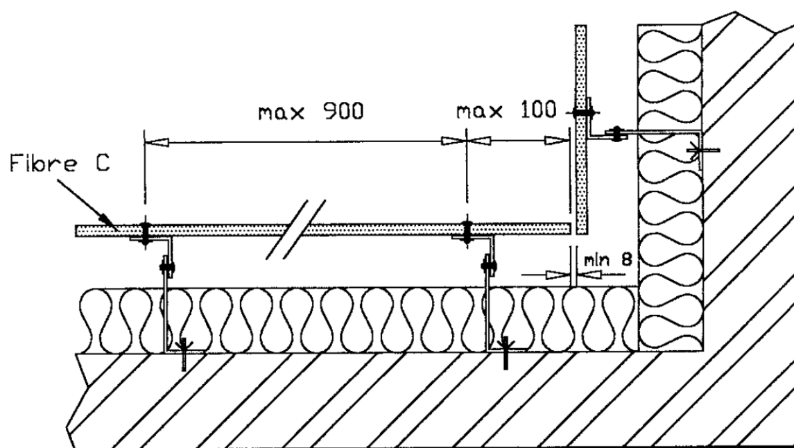
Figure 15 - Angle rentrant
