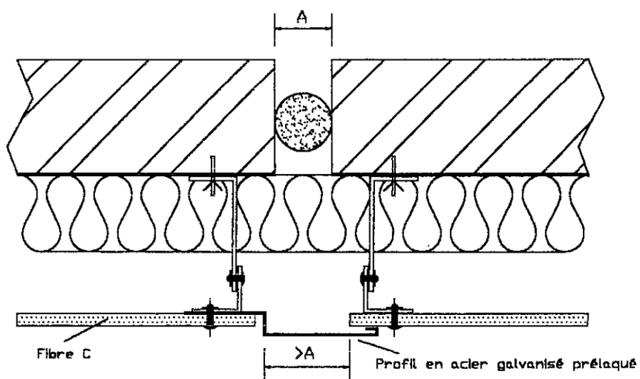
Figure 12 – Joint de dilatation
