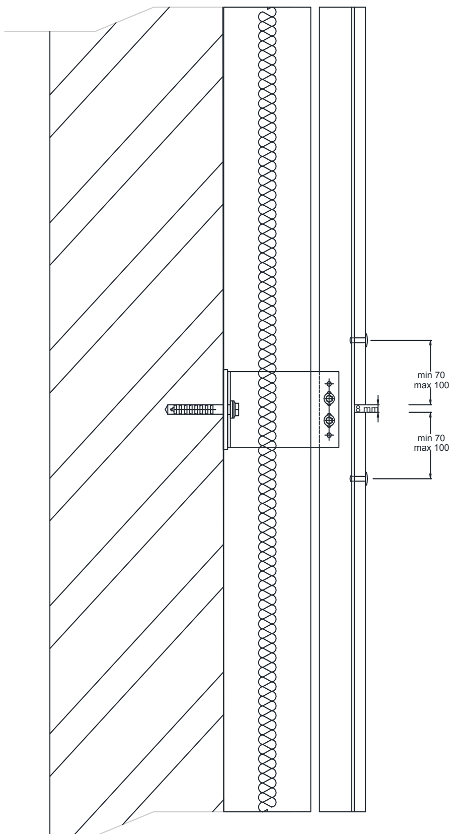
Figure 8 – Joint horizontal
