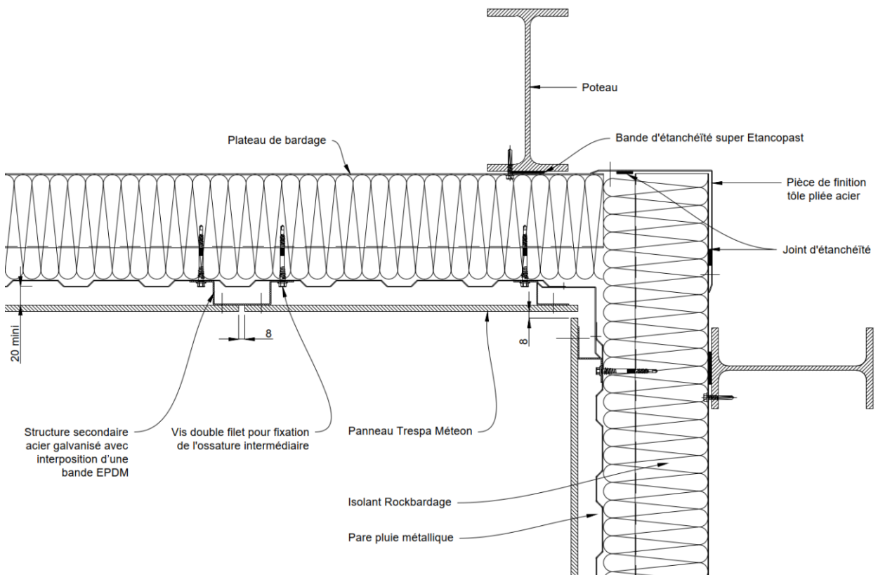
Figure 22 - Angle rentrant
