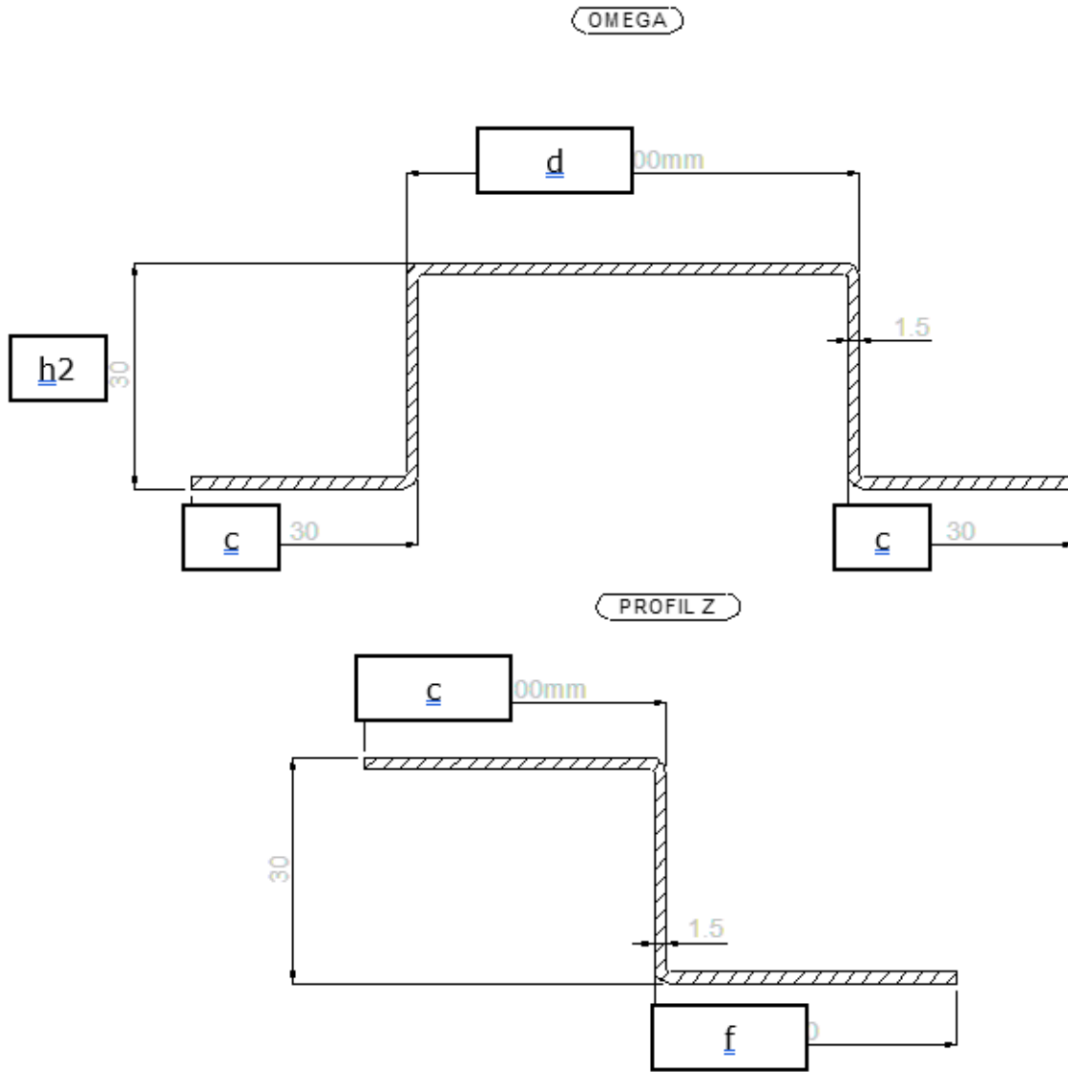
Figure 5 - Profilés
