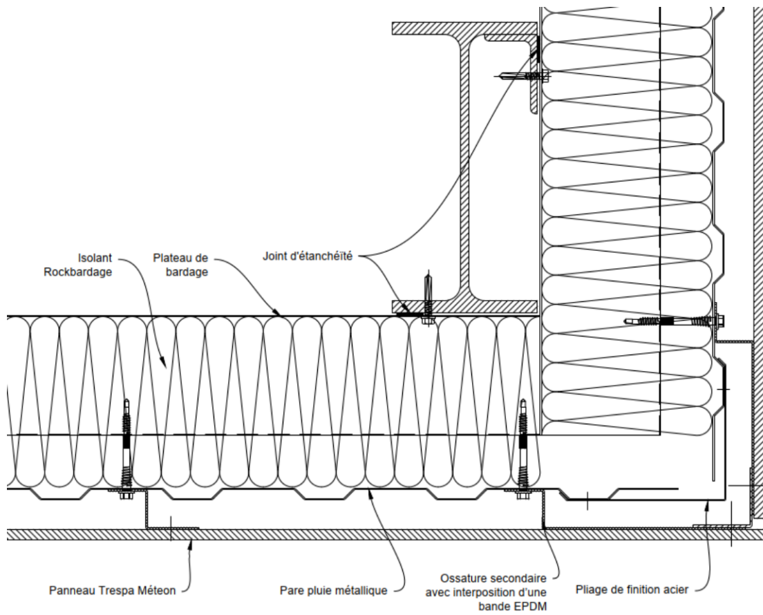
Figure 21 - Angle sortant
