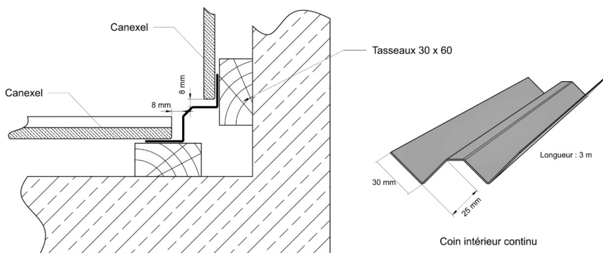
Figure 10 – Angle rentrant
