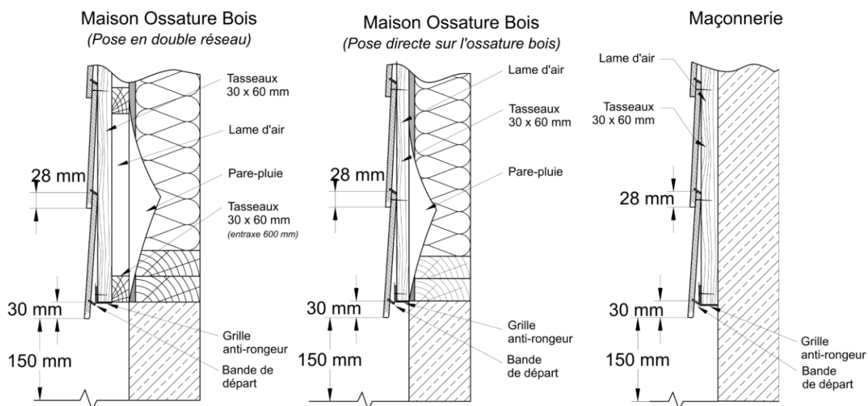
Figure 4 – Pose Horizontale CED'R TEX® ≤ 400 mm
