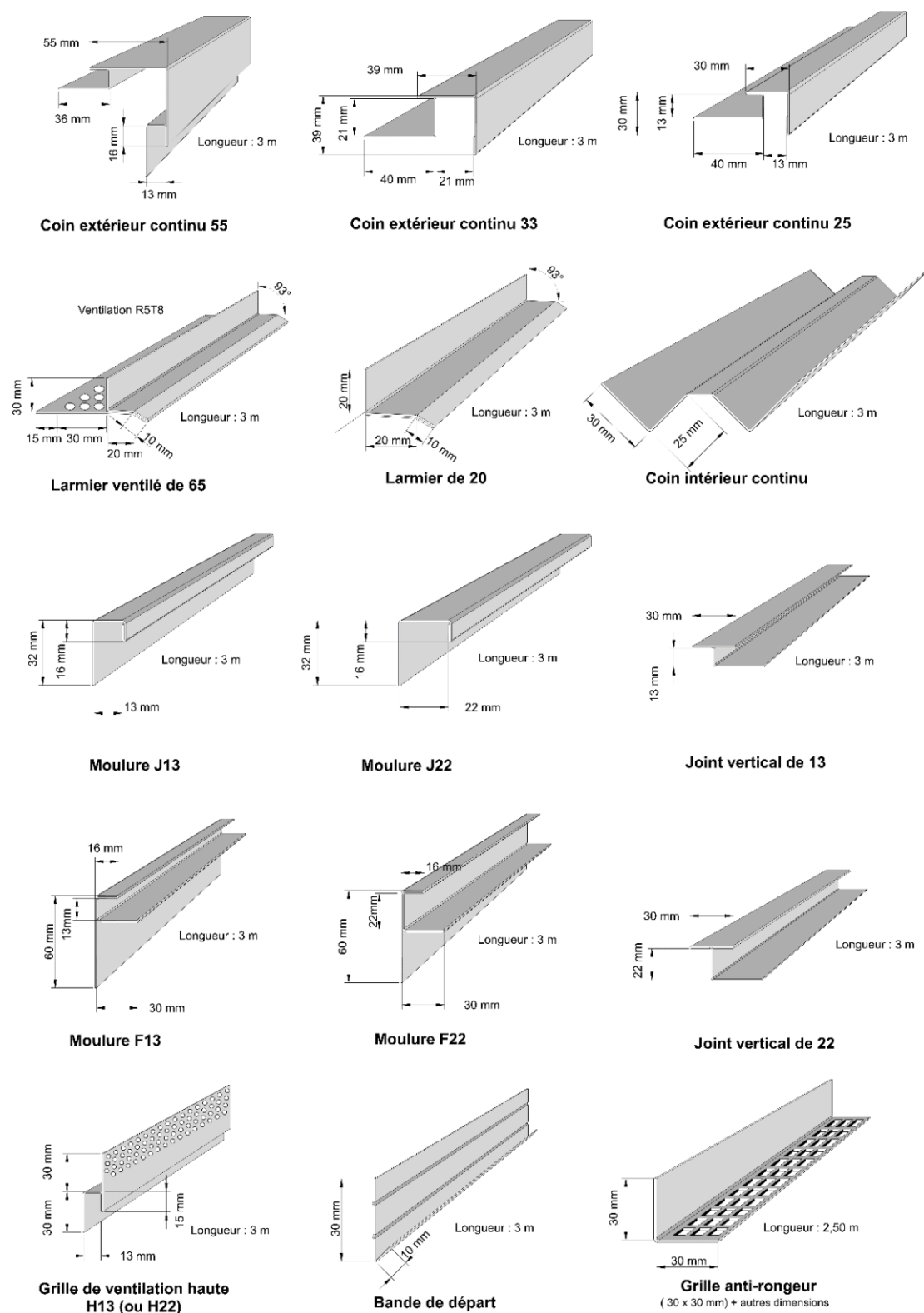
Figure 3 – Accessoires CANEXEL®
