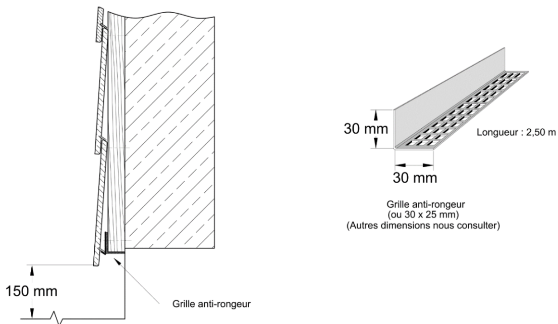
Figure 13 – Grille anti-rongeur
