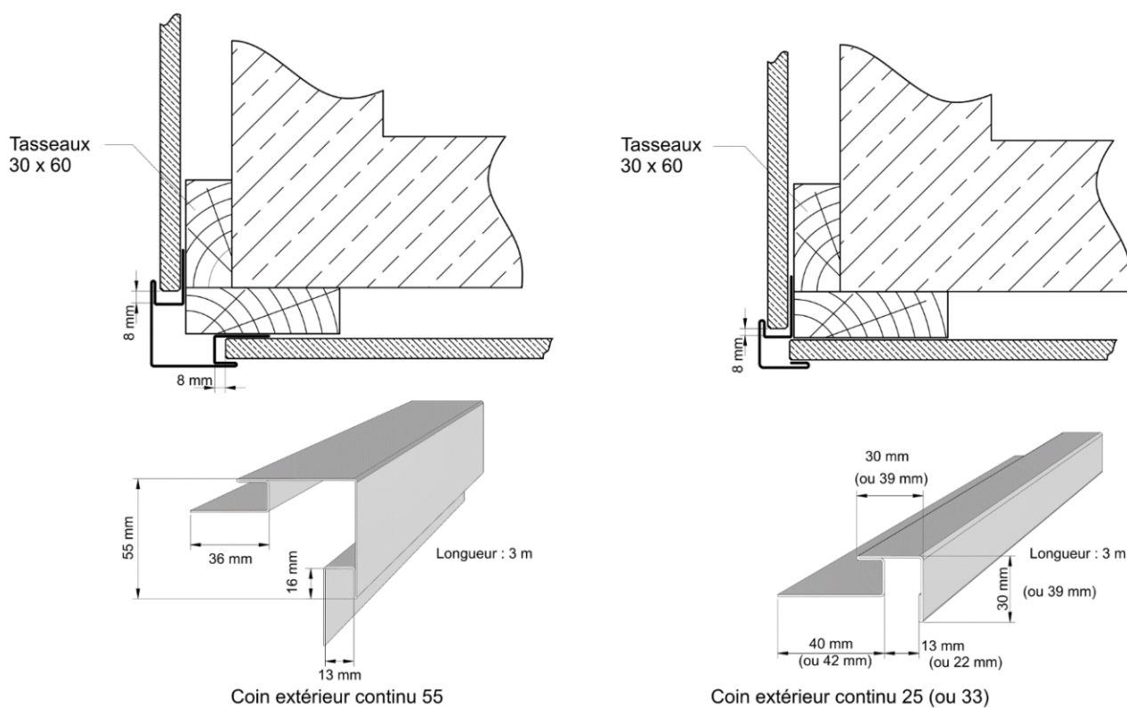
Figure 9 – Angle sortant
