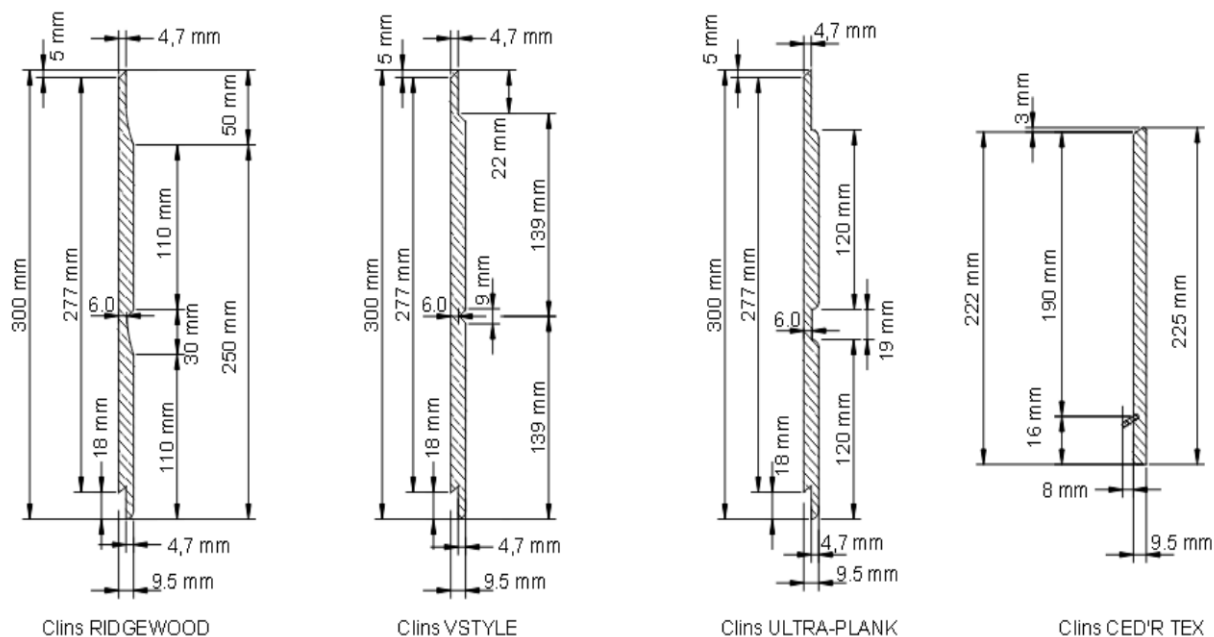
Figure 1 – Clins CANEXEL®
