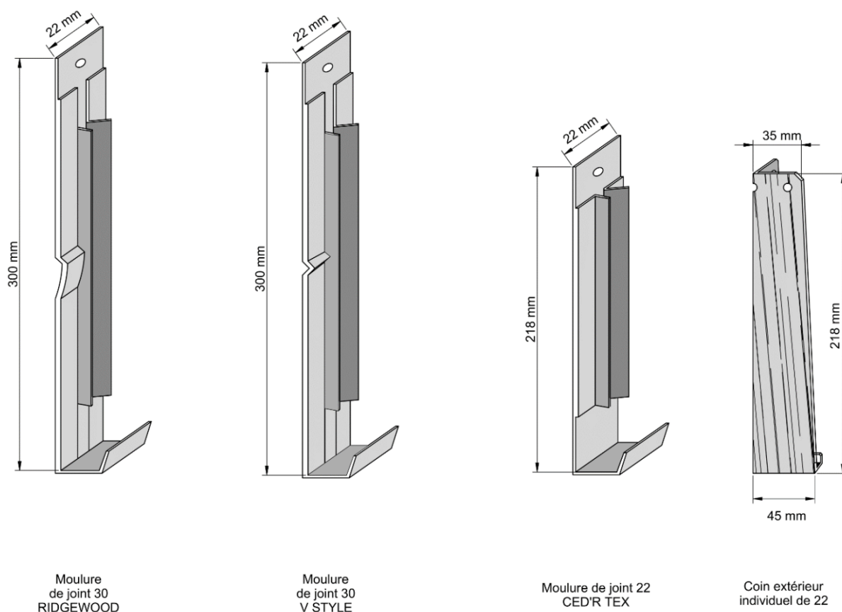
Figure 2 – Accessoires CANEXEL®
