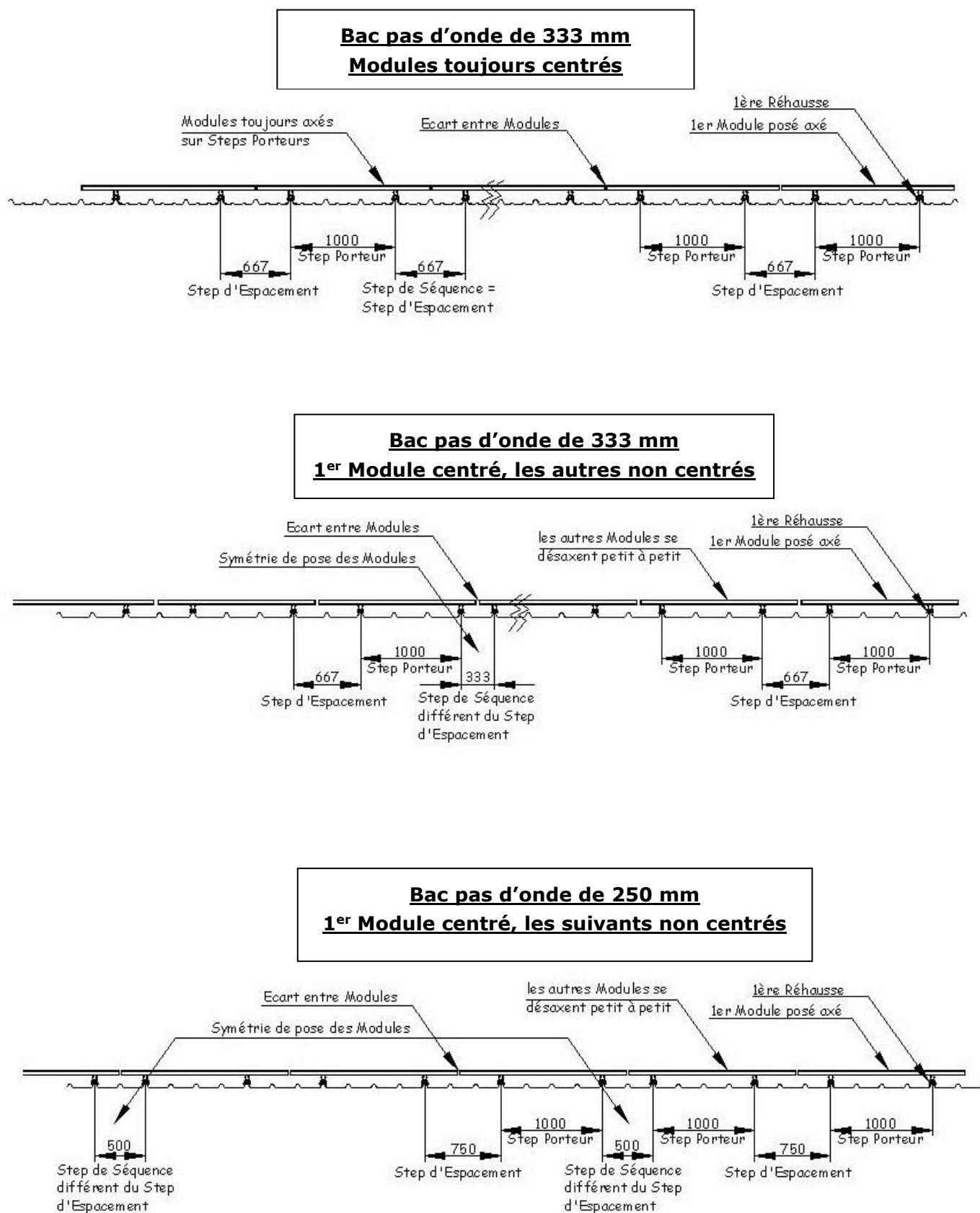
Figure 22 – Calepinage des rails
