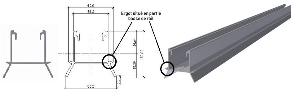
Figure 9 – Rails
