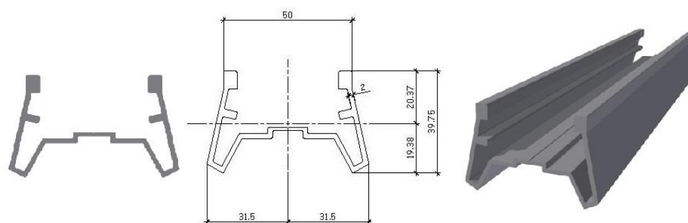
Figure 10 – Éclisses
