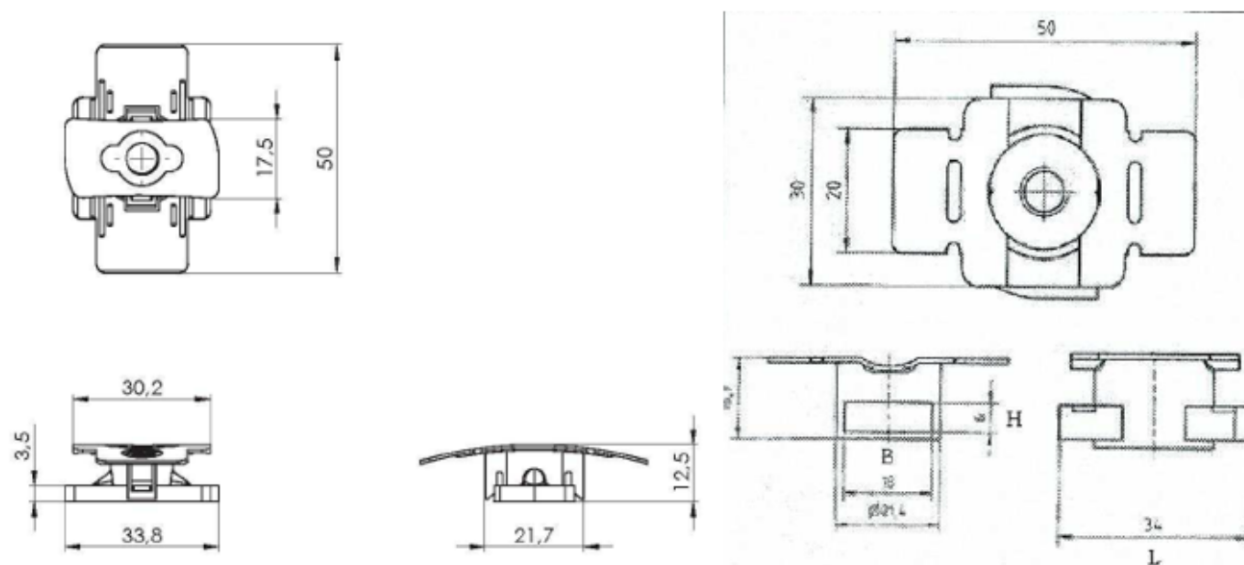
Figure 10 – Serreurs
