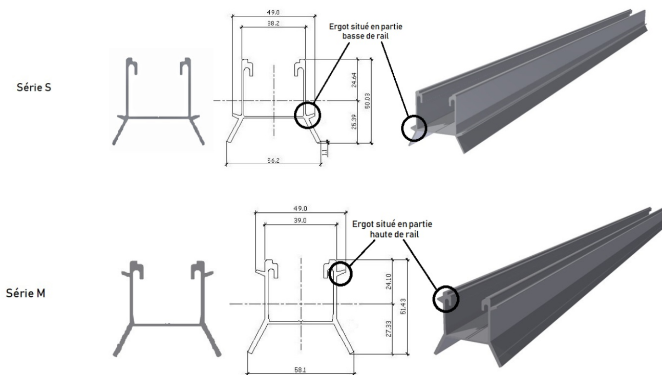
Figure 7 – Joints des rehausses
