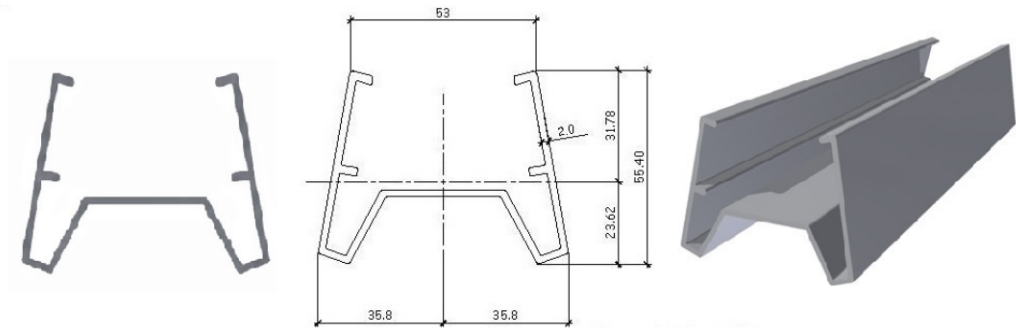
Figure 9 – Éclisses
