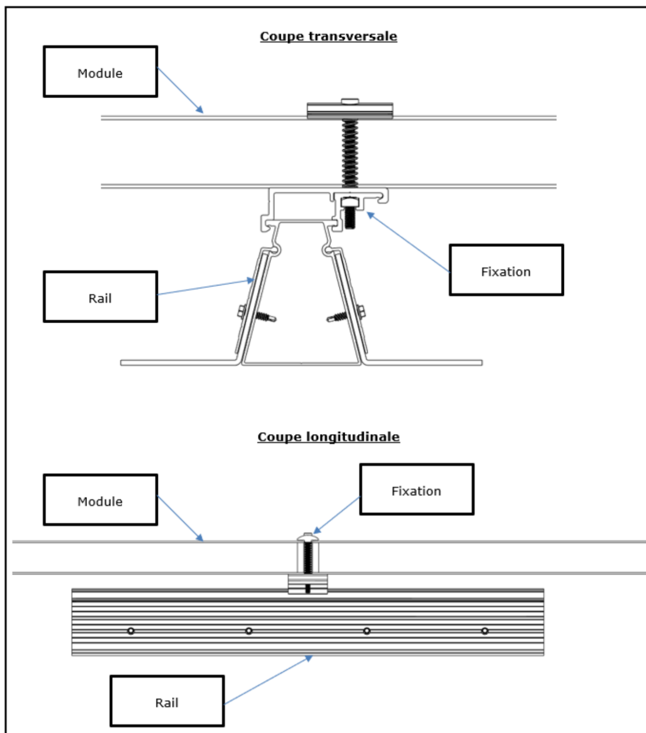
Figure 32 - Assemblage rail / fixation / module
