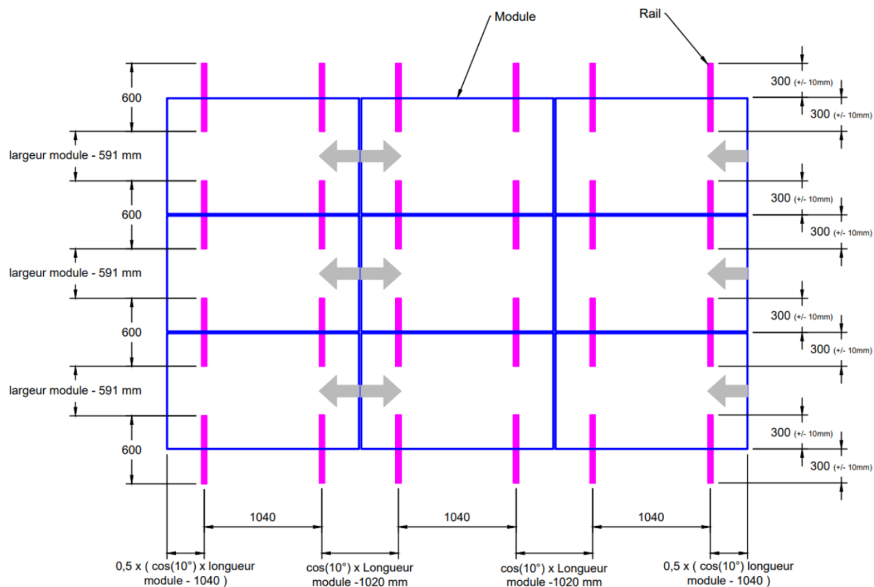
Figure 37 - Implantation des rails / modules double shed
