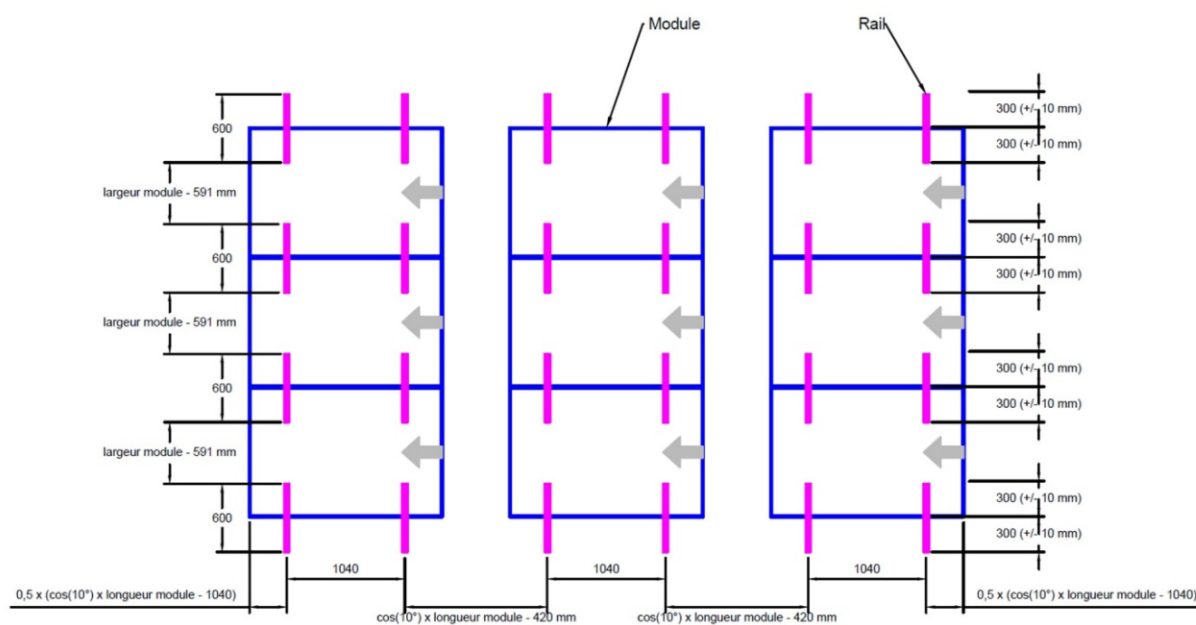
Figure 36 - Implantation des rails / modules simple shed
