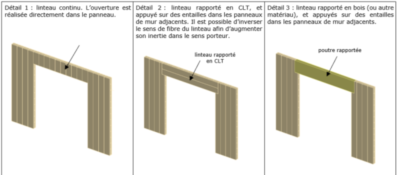
Figure 18: exemples de linteaux
