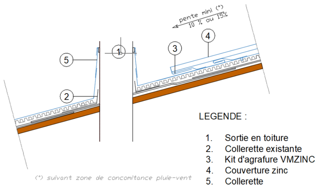
Figure 28 – Pénétration discontinue
