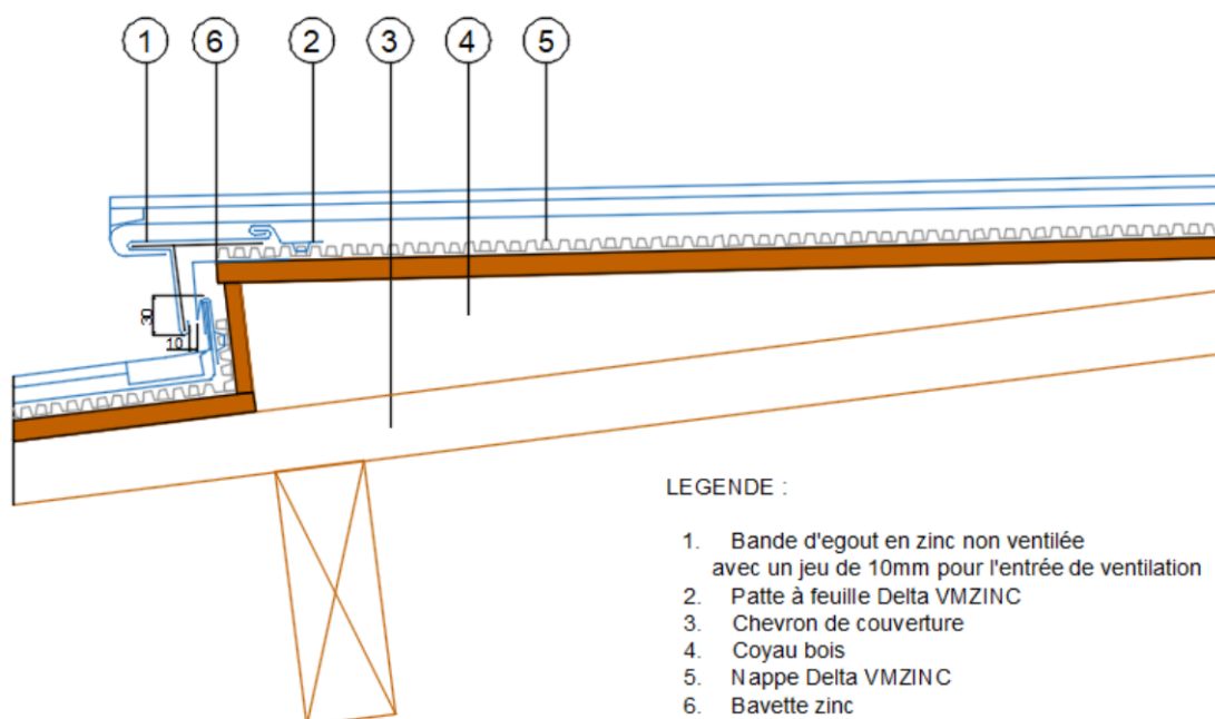
Figure 22 – Ressaut coyau
