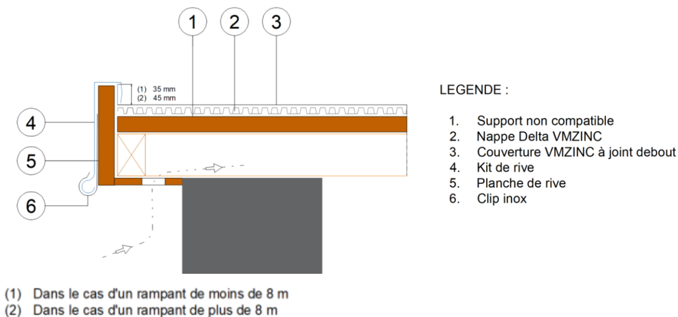
Figure 17 – Rives
