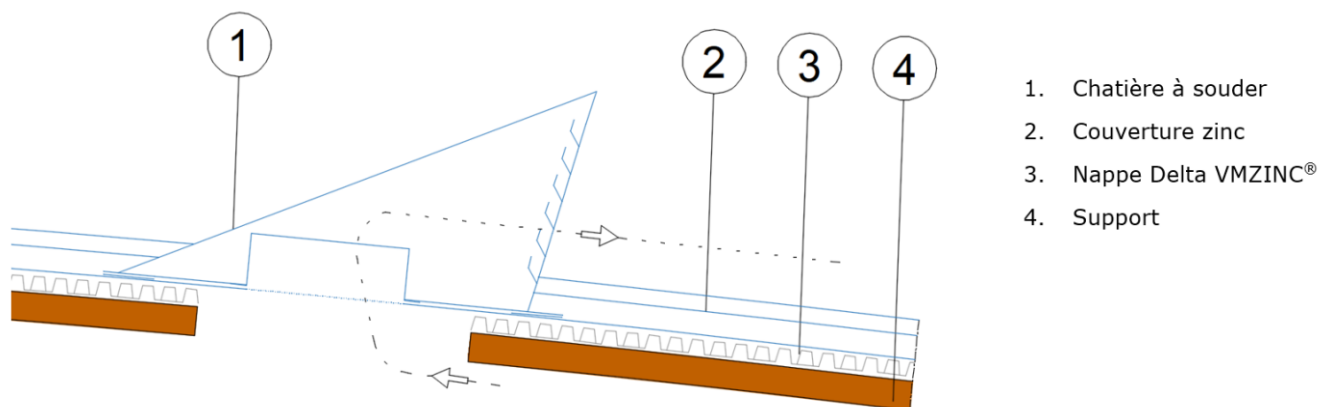
Figure 15 – Chatière
