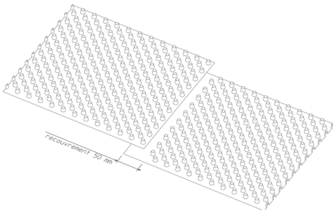
Figure 1 – Nappe Delta VMZINC®
