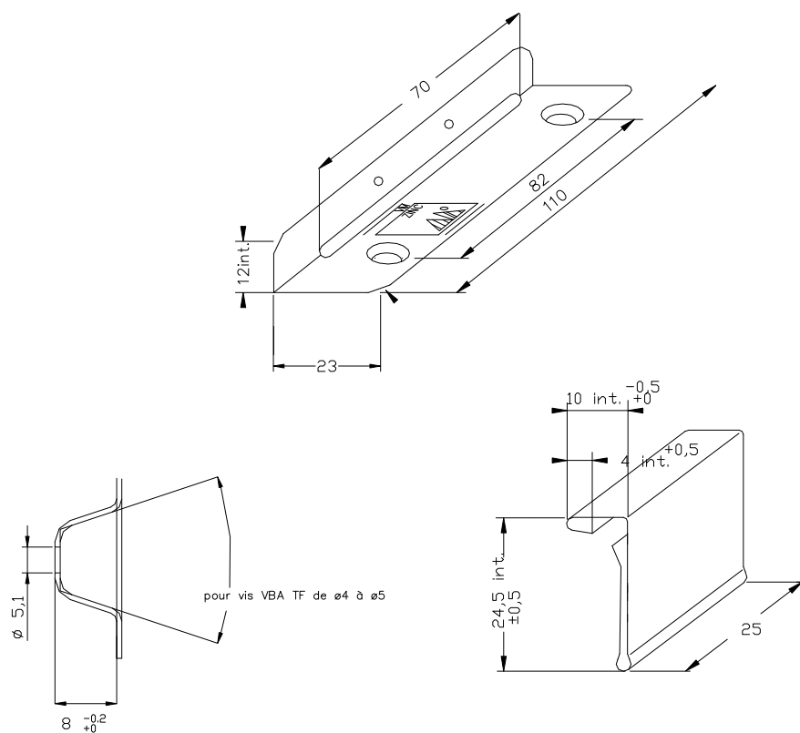
Figure 3 – Patte coulissante Delta VMZINC®
