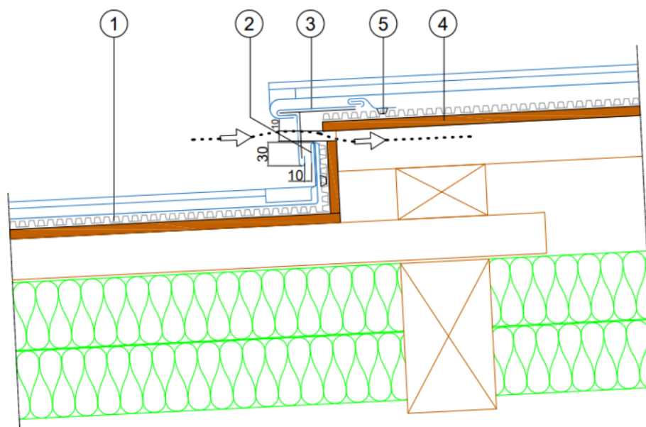
Figure 21 – Ressaut
