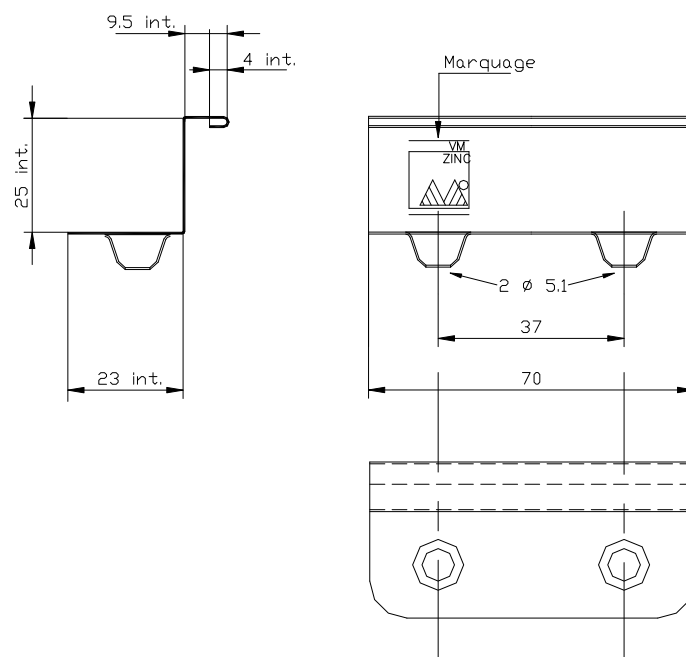
Figure 4 – Patte fixe Delta VMZINC®
