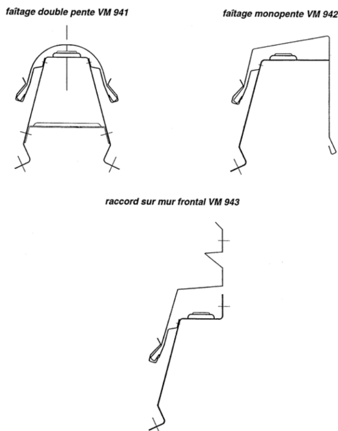
Figure 7 – Faîtages
