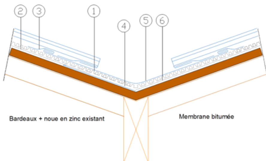
Figure 33 – Noue, pente > 20 %
