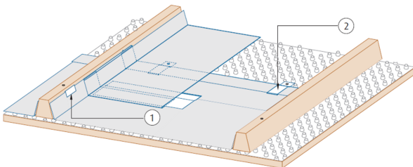
Figure 8 – Fixation des tasseaux
