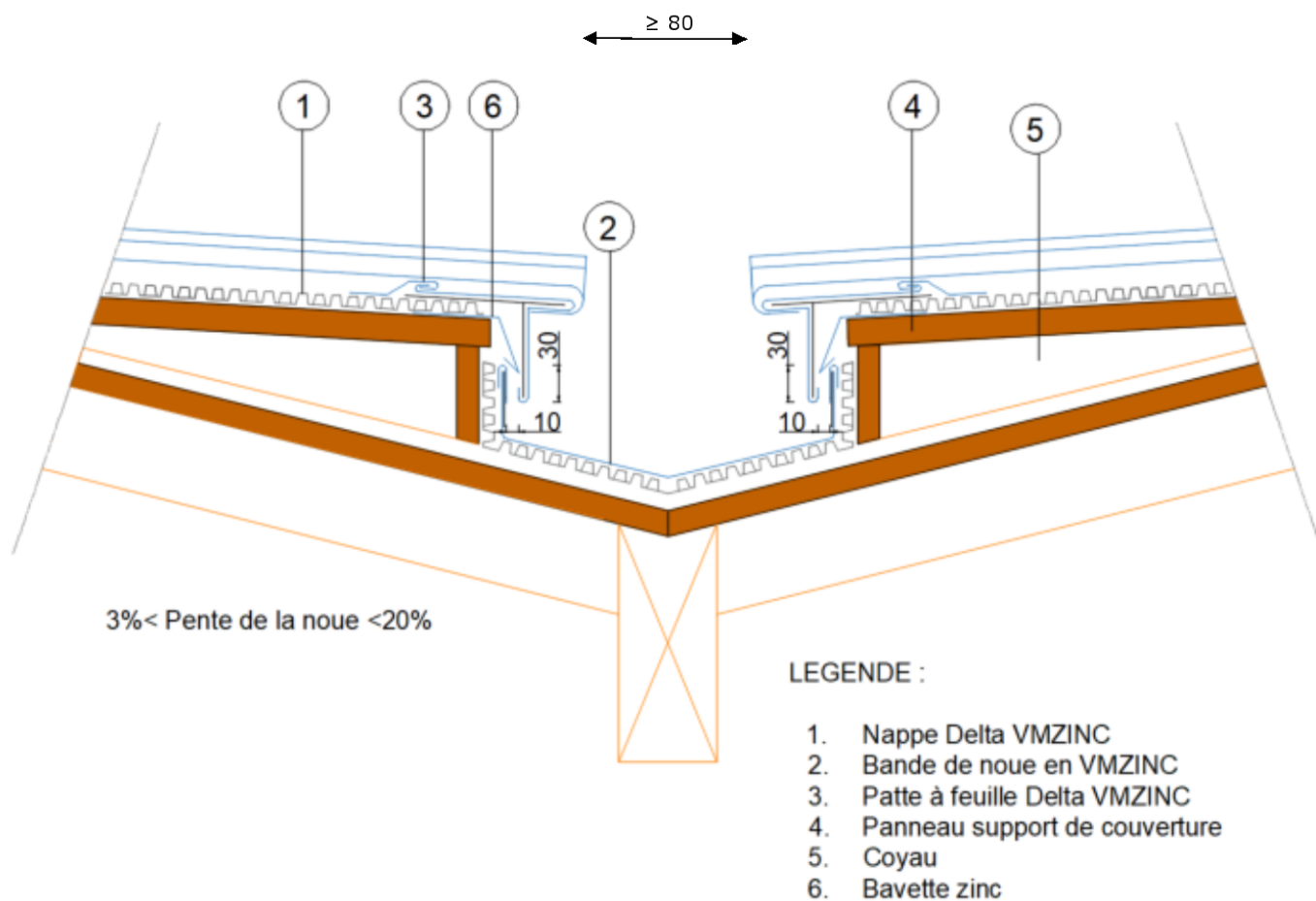
Figure 20 – Noue encaissée
