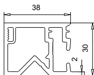
109 461.2 Tapée 38 mm
