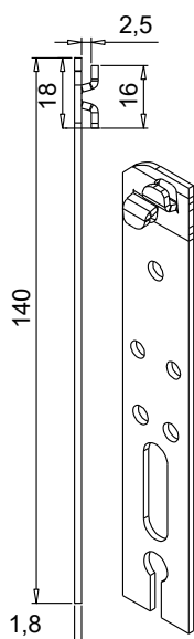
PAC0648 ACIER GALVA
