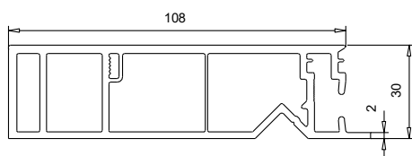
109 463.1 Tapée 108 mm
