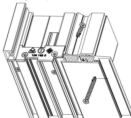
4-Pose tapée ou coulisse tapée 5-Vissages tapée
