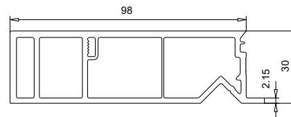
109 463.2 Tapée 98 mm
