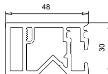
109 461.4 Tapée 48 mm
