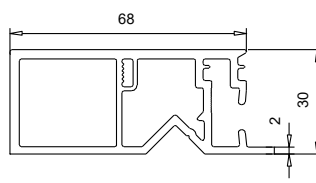
109 462.1 Tapée 68 mm
