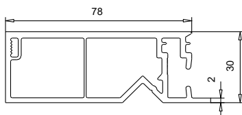
109 463.4 Tapée 78 mm
