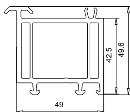
109 445 Profil raccord balcon
