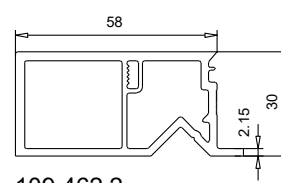
109 462.2 Tapée 58 mm
