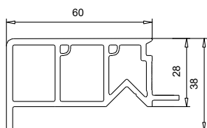
109 414 Tapée 60 mm
