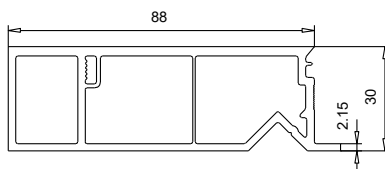
109 463.3 Tapée 88 mm
