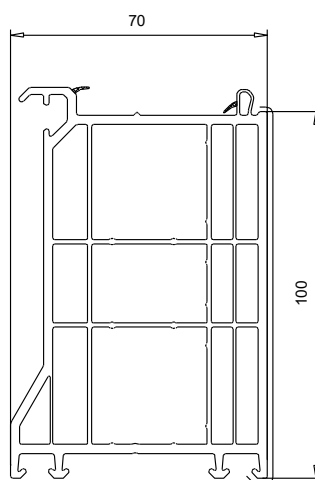
109 660 Profil raccord balcon
