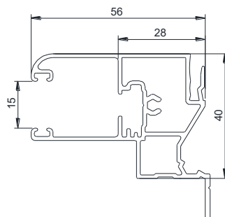
COULISSE RENOVATION 56 x 40 PIED 22 ALUMINIUM 0322
