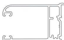
COULISSE ALUMINIUM 45 0338
