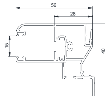
COULISSE RENOVATION 56 x 40 T ALUMINIUM 0324
