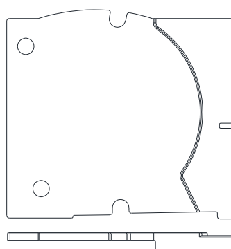
Isolation embout - coffre 195 6 mm D 11171699
