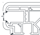
coulisse tapée 45
