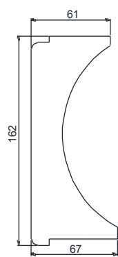
FACADE 195 28 kg/m3 : 11175499
