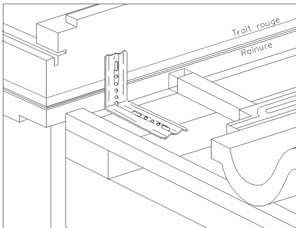
RACCORDEMENT EL/EW
