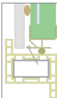
Rail PVC standard
