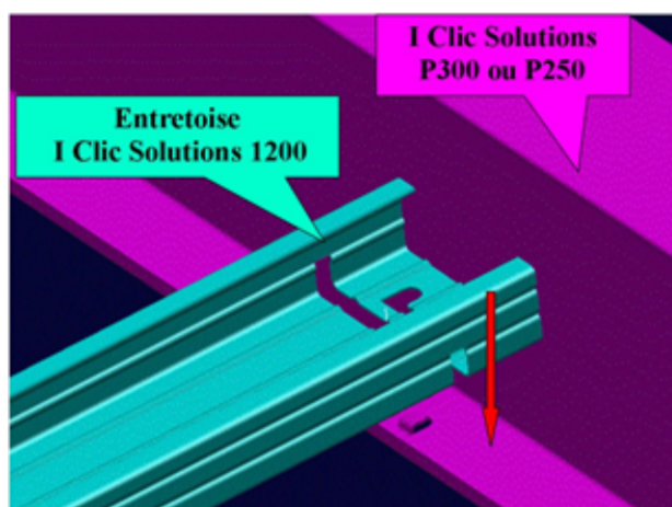
Figure 3-1 : pose
