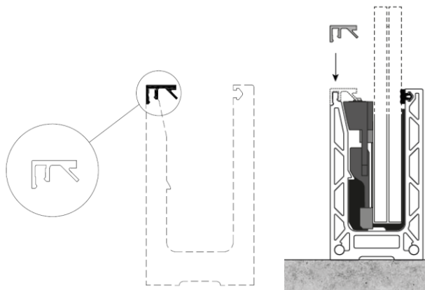
Figure 6 – Capot de finition
