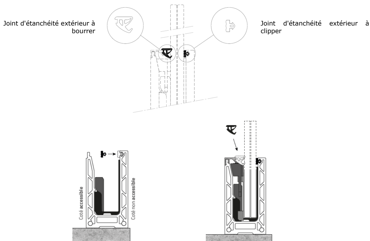
Figure 5 – Garnitures d'étanchéité
