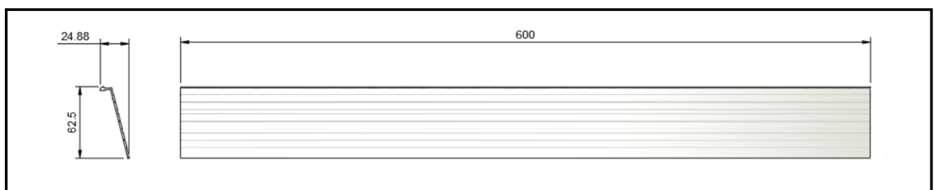
Figure 7 - Ailette
