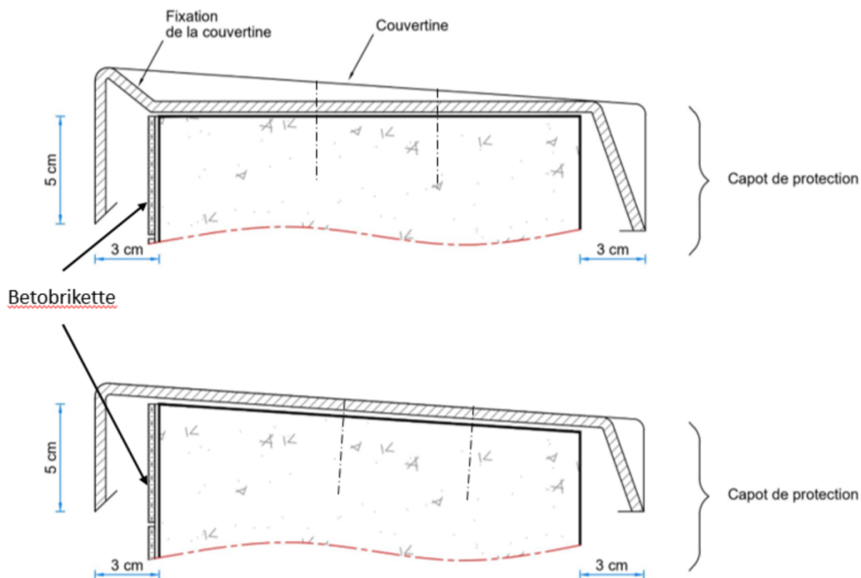
Figure 4 - Traitement couverture
