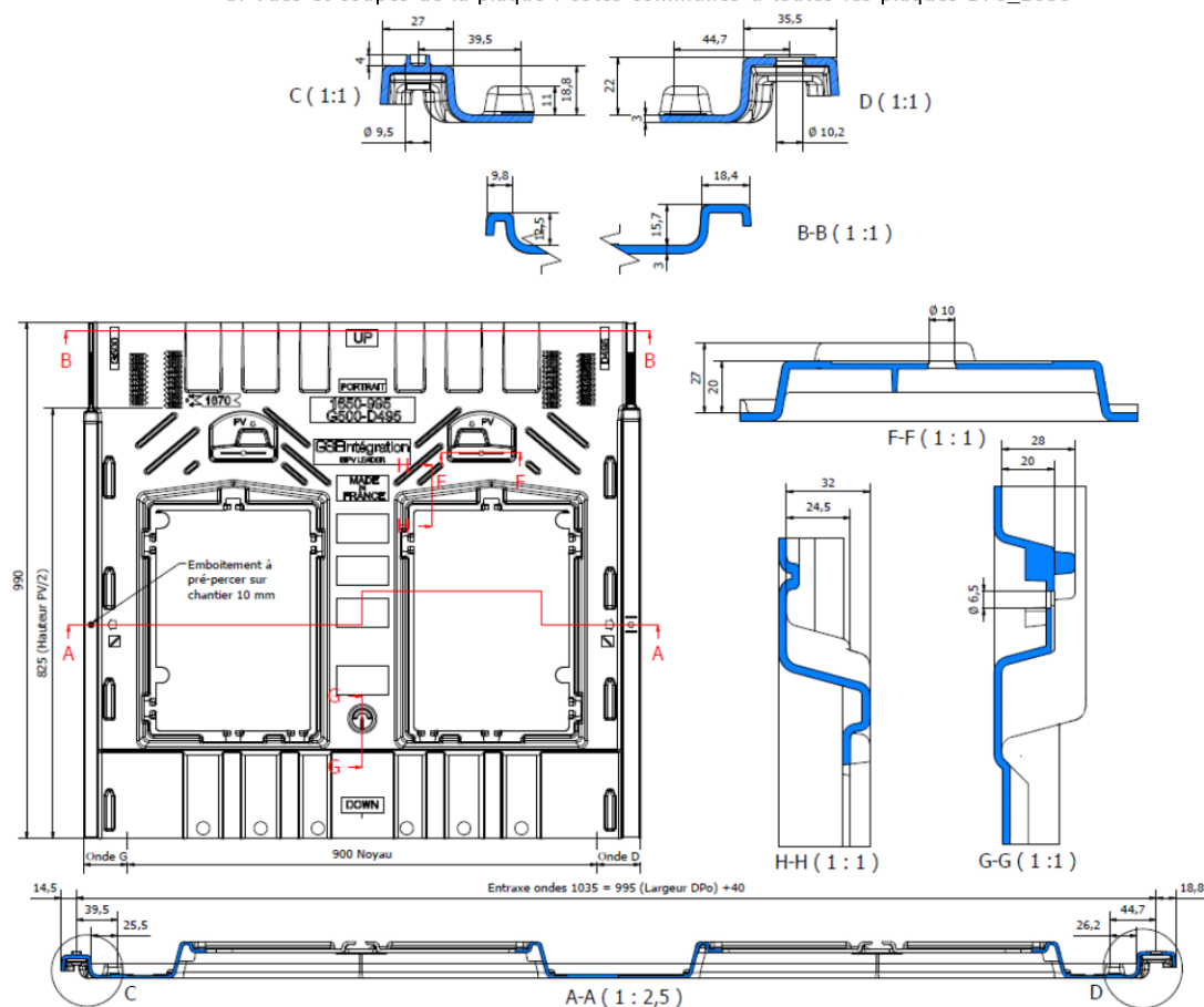
Figure 3 – Plaque polypropylène
