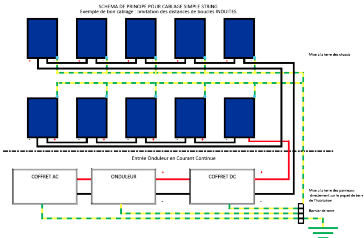
Figure 16 – Principe de câblage
