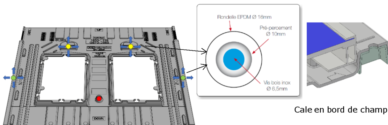
Figure 22 – Pose de plaques polypropylène
