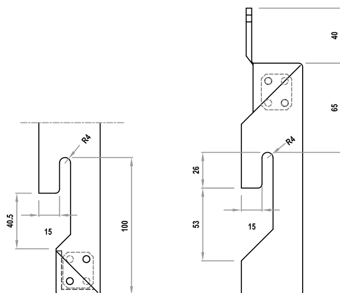
Figure 2b – Cassette 4 plis – type 1
