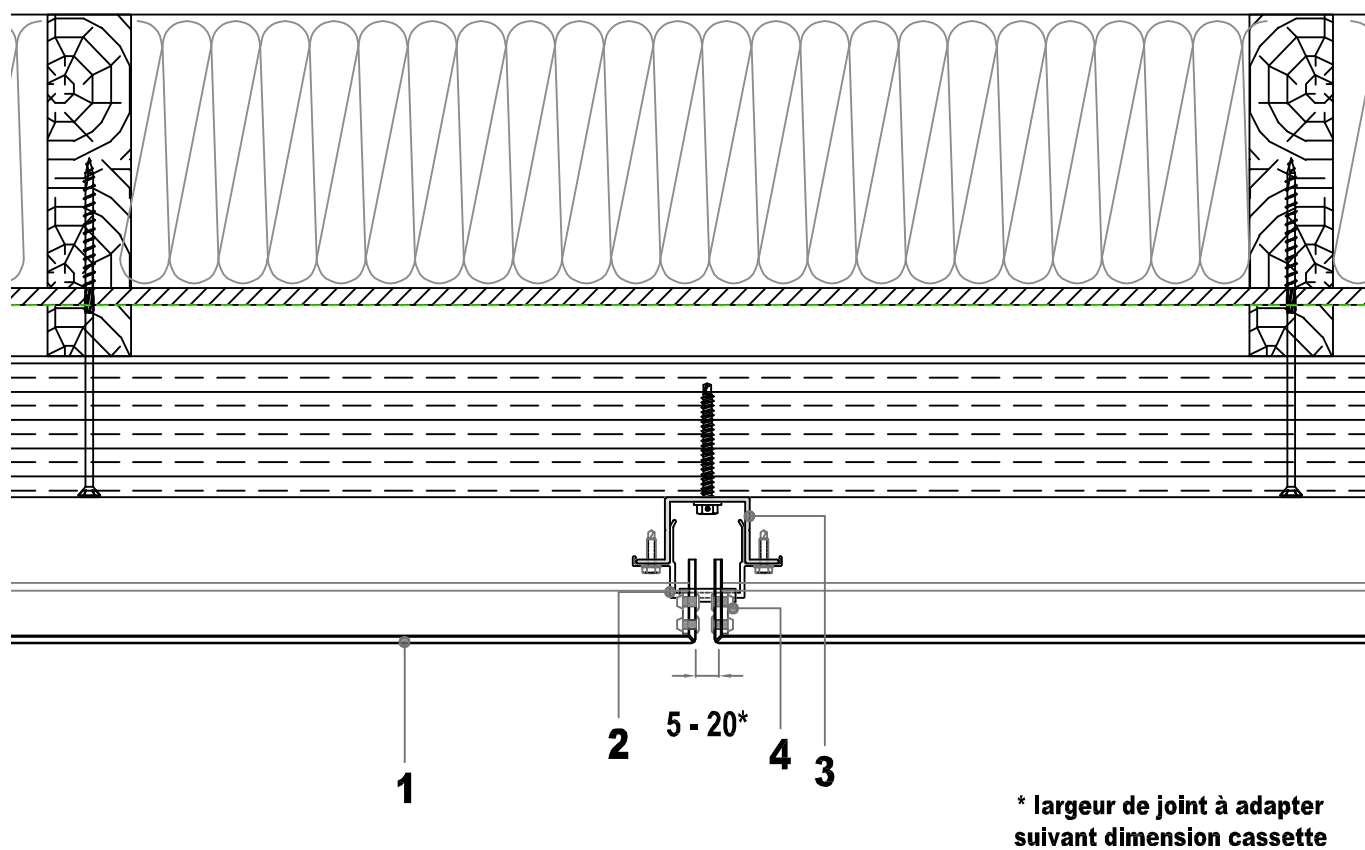
Figure 9b – Pose sur COB/CLT - Joint vertical - coupe horizontale – lisse horizontale bois
