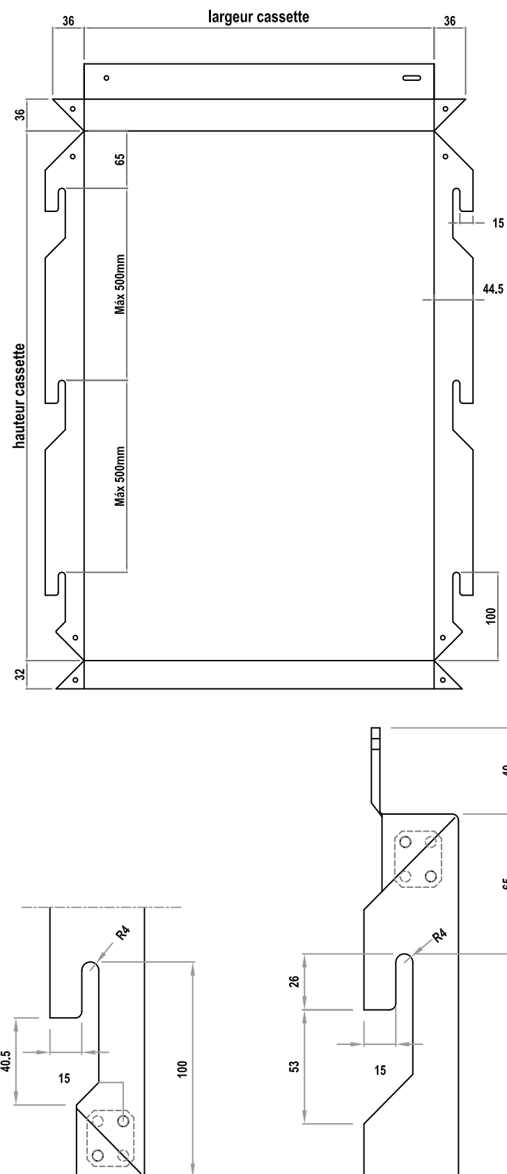
Figure 2a – Cassette 3 plis
