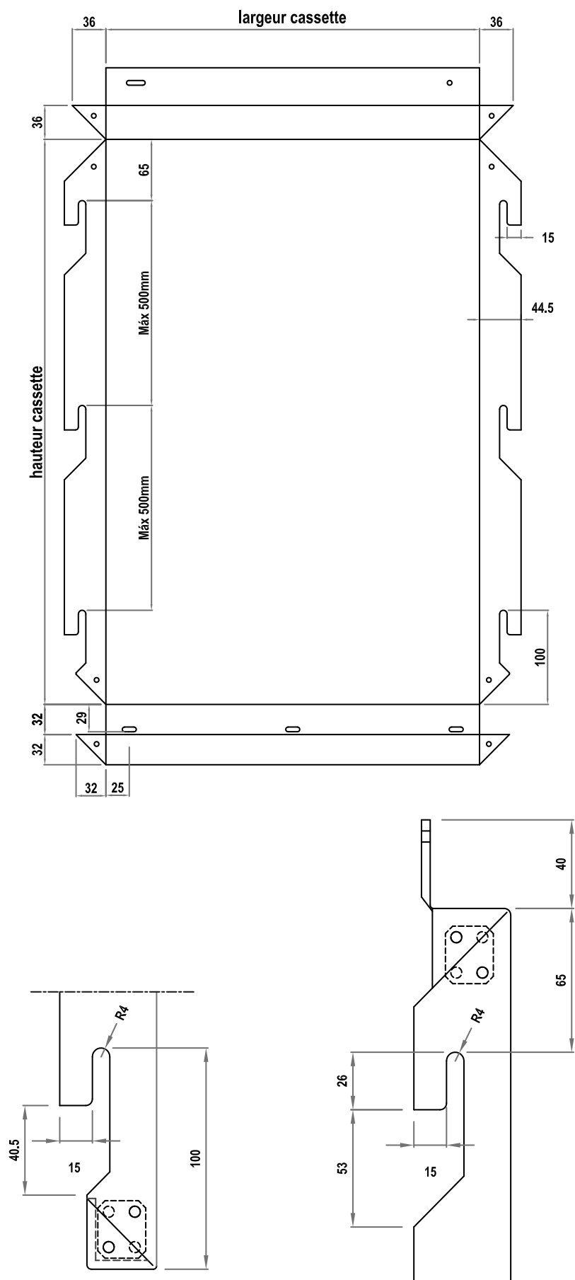
Figure 2c – Cassette 4 plis – type 2
