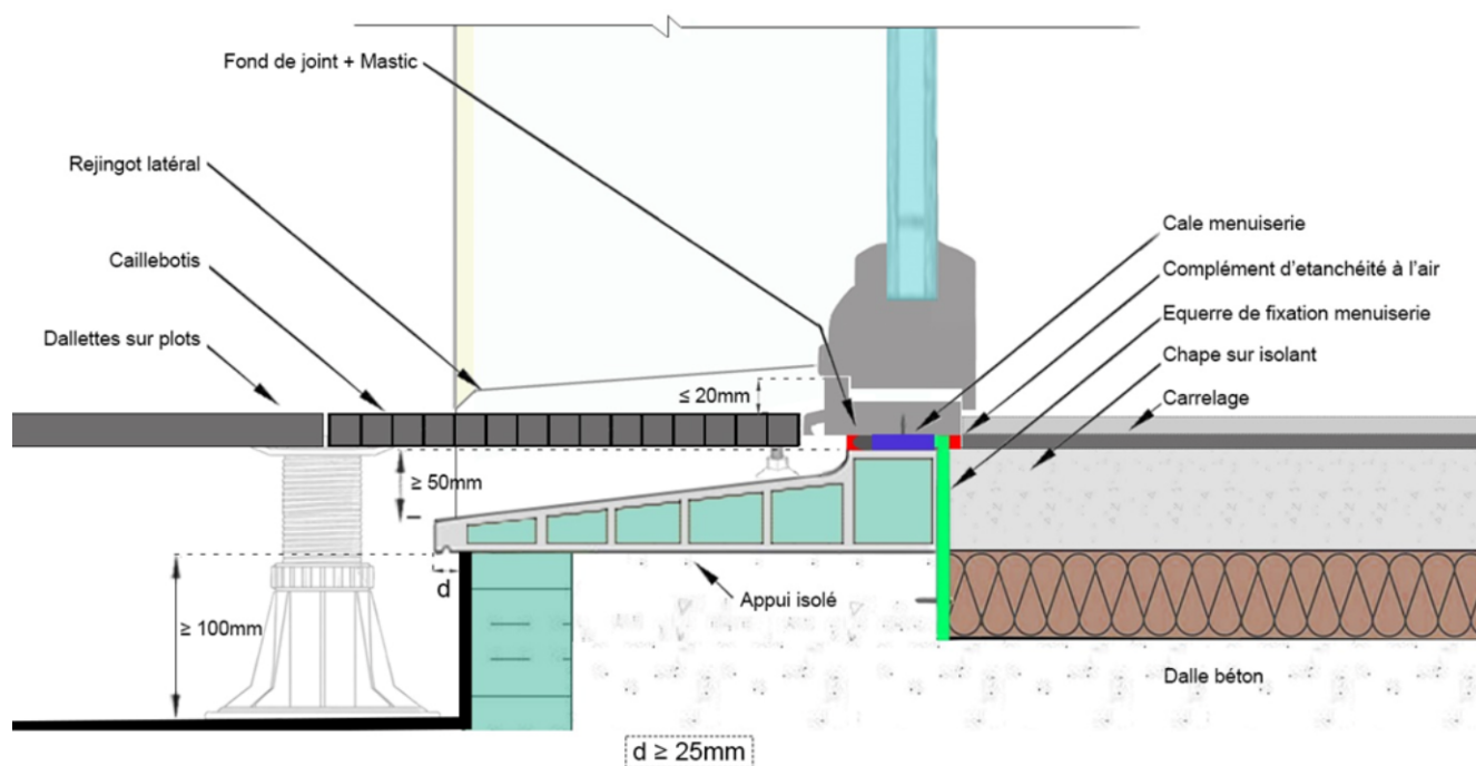
Figure 29 - Seuil PMR
