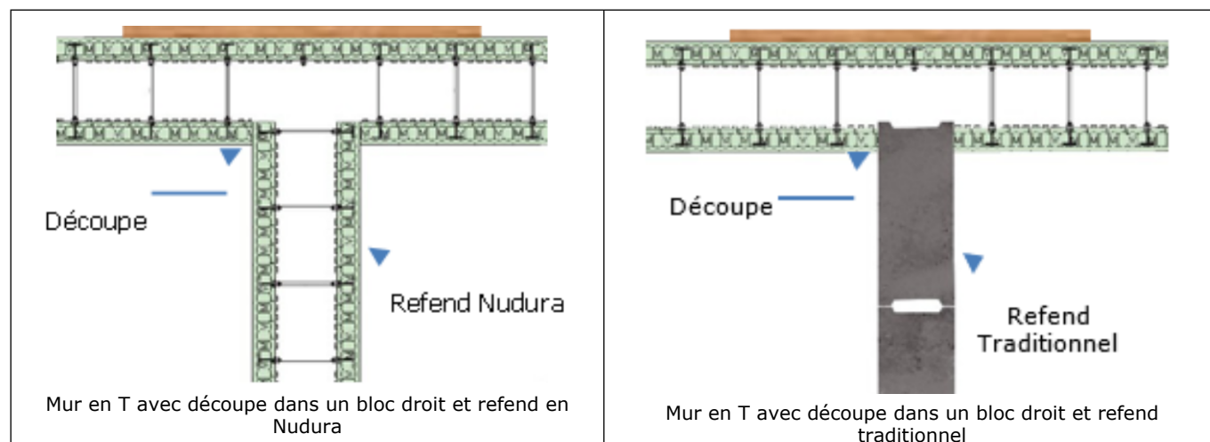
Figure 17 - Jonctions Mur Nudura / Refend
