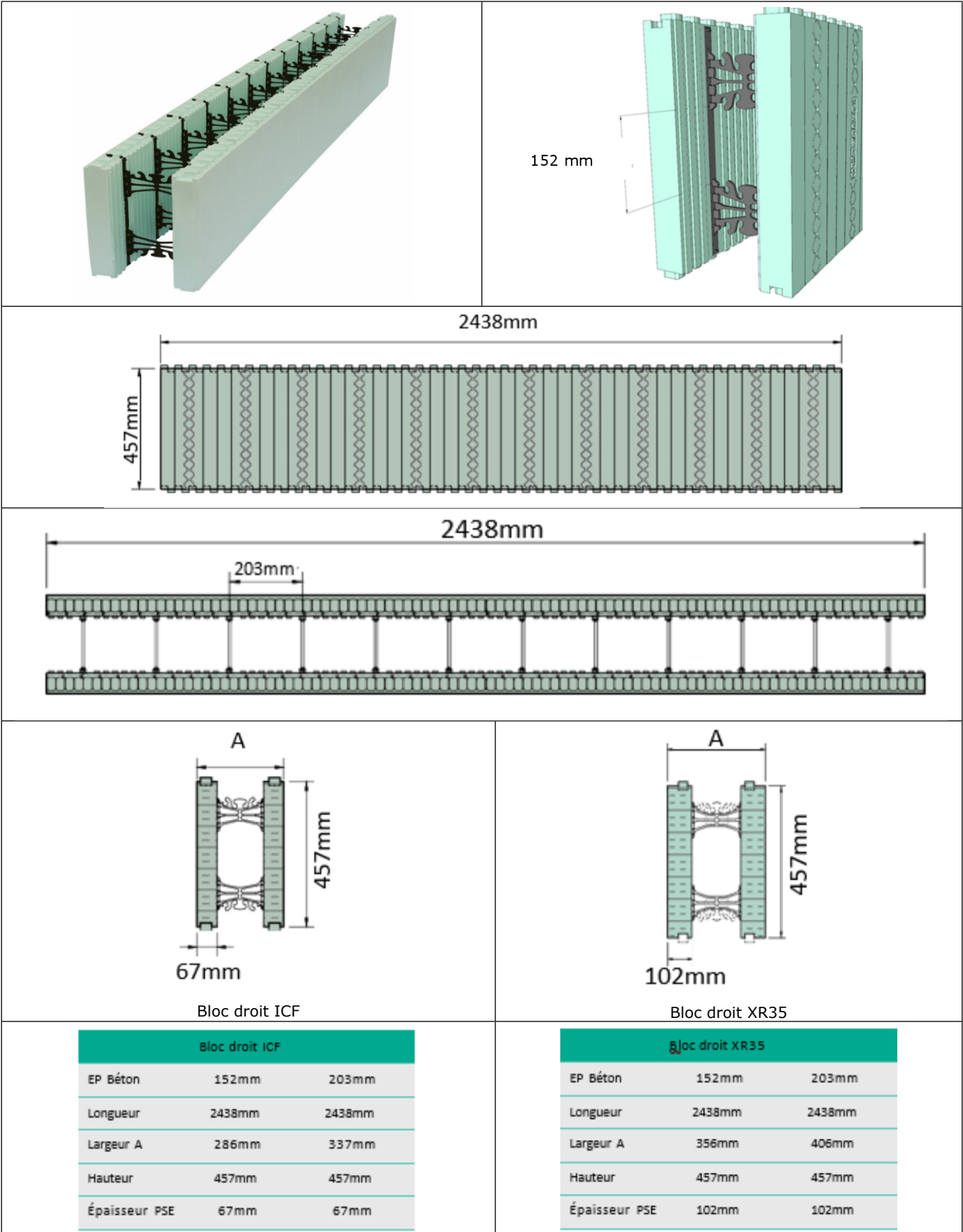
Figure 5 - Blocs droits Nudura
