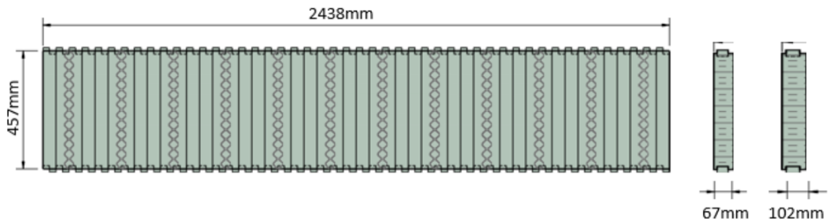
Figure 1 - Planelle Nudura
