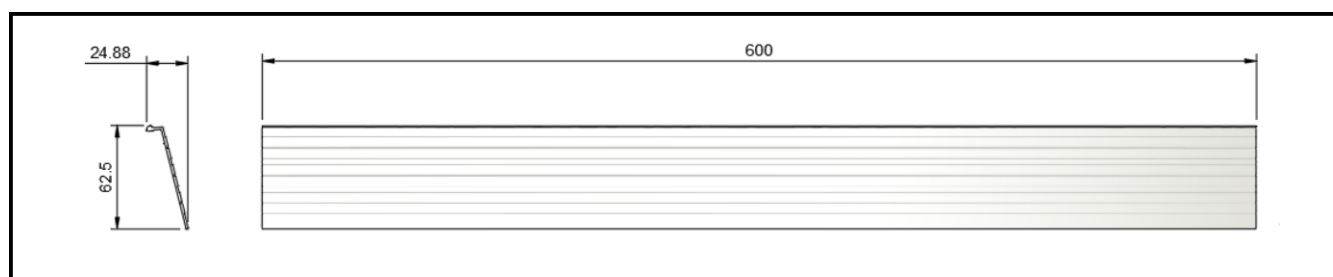
Figure 7 - Ailette
