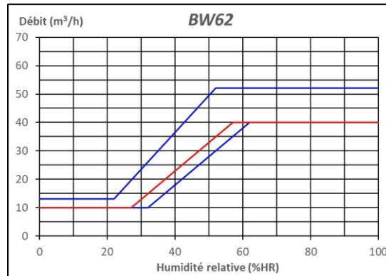
Figure 43 – BW62 (10-40/30 m³/h, 27-57%HR)
