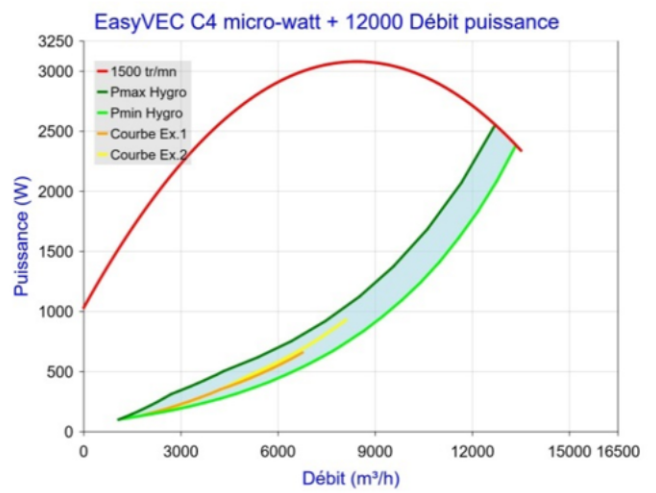
Figure 68 - EasyVEC C4 micro-watt + 12000 (sans T.Flow Hygro+/T.Flow Nano ou T.Flow 105 / T.Flow 180)
