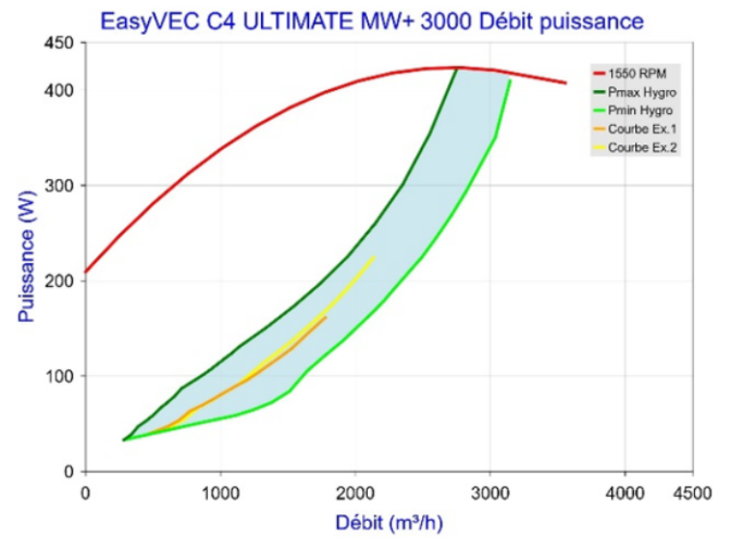
Figure 104 - EasyVEC C4 ULTIMATE MW+ 3000 (sans T.Flow Hygro+/T.Flow Nano ou T.Flow 105 / T.Flow 180)
