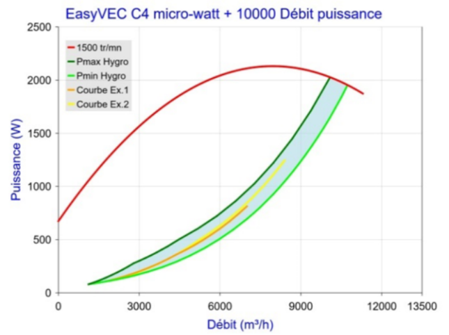
Figure 67 - EasyVEC C4 micro-watt + 10000 (sans T.Flow Hygro+/T.Flow Nano ou T.Flow 105 / T.Flow 180)
