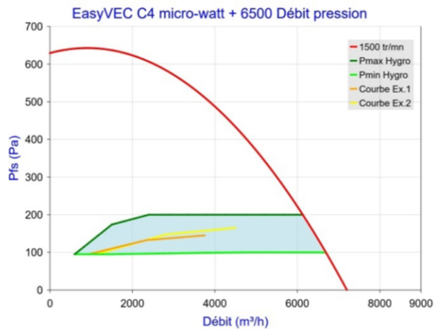
Figure 65 - EasyVEC C4 micro-watt + 6500 (sans T.Flow Hygro+/T.Flow Nano ou T.Flow 105 / T.Flow 180)
