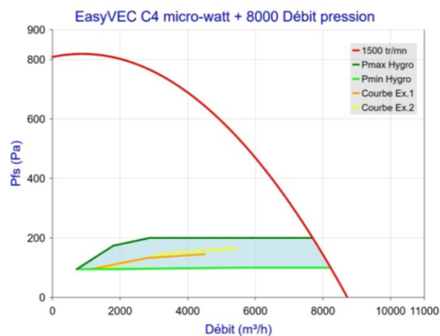
Figure 66 - EasyVEC C4 micro-watt + 8000 (sans T.Flow Hygro+/T.Flow Nano ou T.Flow 105 / T.Flow 180)
