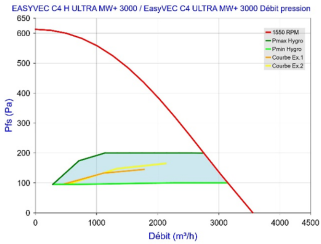
Figure 88 - EasyVEC C4 (H) ULTRA MW+ 3000 (sans T.Flow Hygro+/T.Flow Nano ou T.Flow 105 / T.Flow 180)
