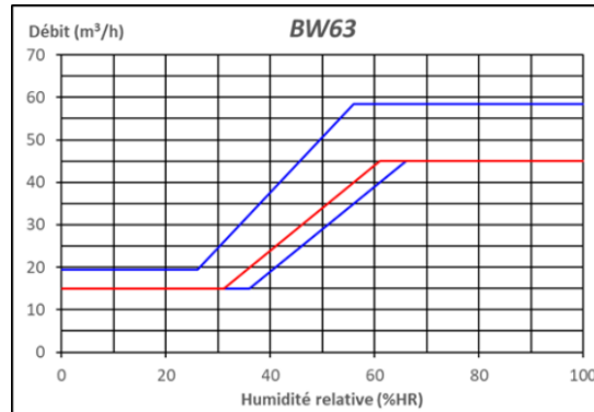
Figure 44 – BW63 (15-45/45 m³/h, 31-61%HR)
