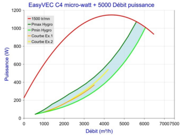
Figure 64 - EasyVEC C4 micro-watt + 5000 (sans T.Flow Hygro+/T.Flow Nano ou T.Flow 105 / T.Flow 180)
