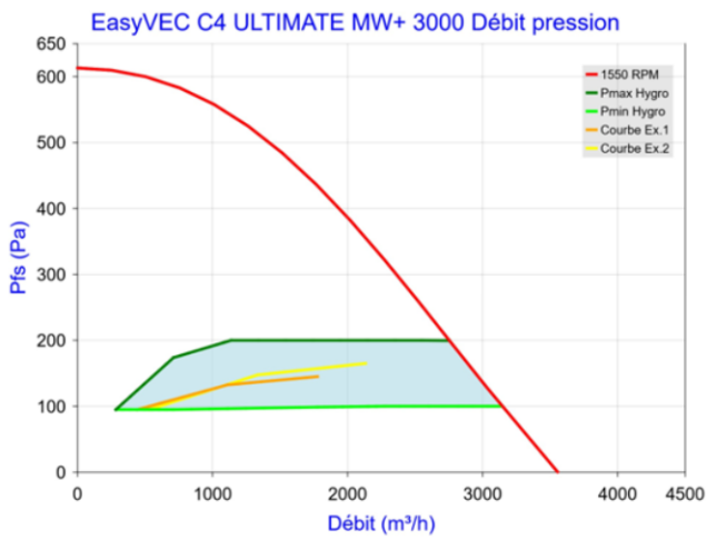
Figure 104 - EasyVEC C4 ULTIMATE MW+ 3000 (sans T.Flow Hygro+/T.Flow Nano ou T.Flow 105 / T.Flow 180)
