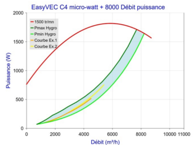
Figure 66 - EasyVEC C4 micro-watt + 8000 (sans T.Flow Hygro+/T.Flow Nano ou T.Flow 105 / T.Flow 180)
