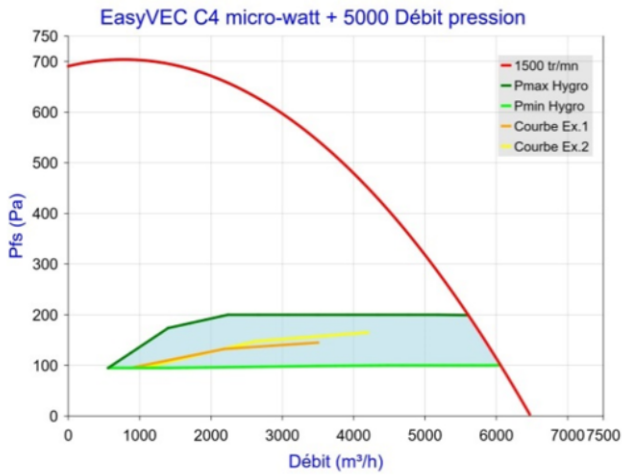
Figure 64 - EasyVEC C4 micro-watt + 5000 (sans T.Flow Hygro+/T.Flow Nano ou T.Flow 105 / T.Flow 180)
