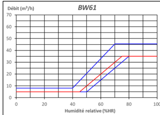
Figure 42 – BW61 (5-35/30 m³/h, 45-75%HR)
