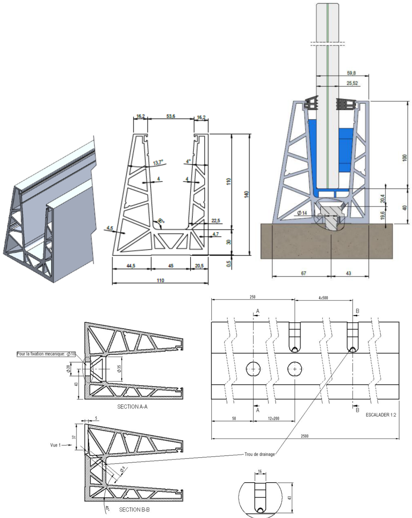
Figure 6 – GlassFit SV-1801 RX Top dimensions
