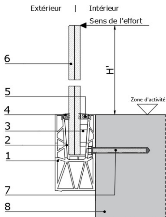
Figure 4 – GlassFit SV-1802 Side – Montage latéral
