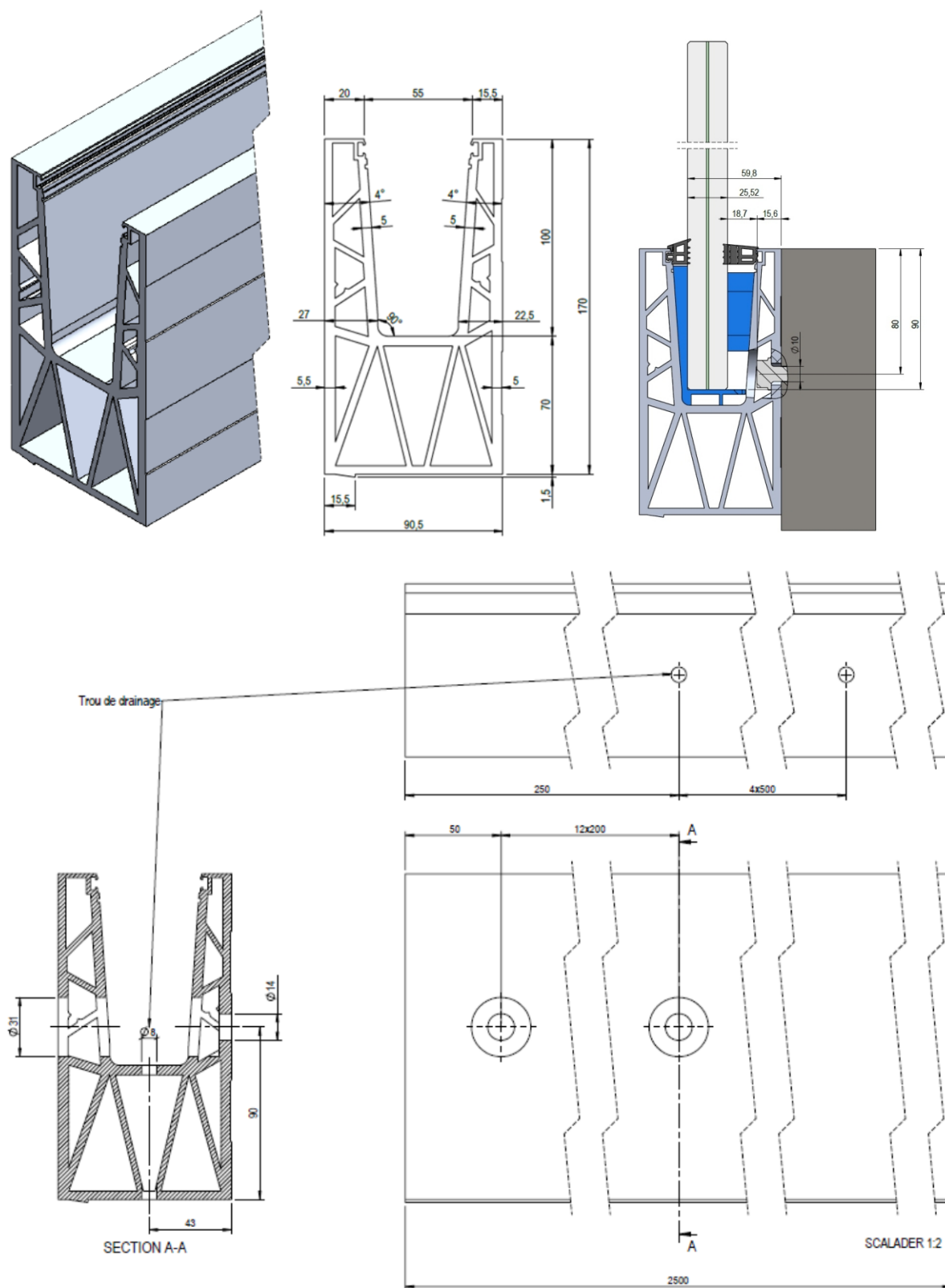
Figure 7 – GlassFit SV-1802 Side dimensions
